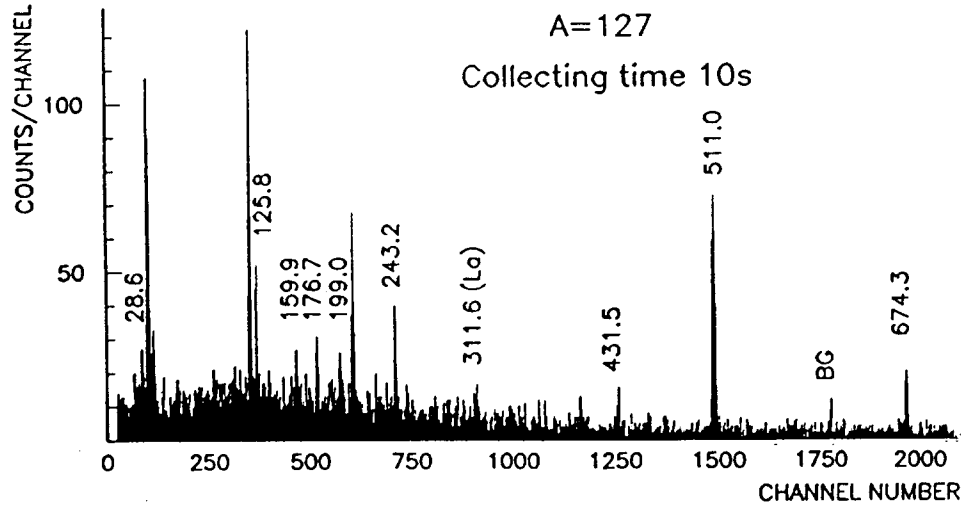
Figure 5 : \beta -gated \gamma spectrum measured at mass A=127 with 10s collection-and counting-time.
