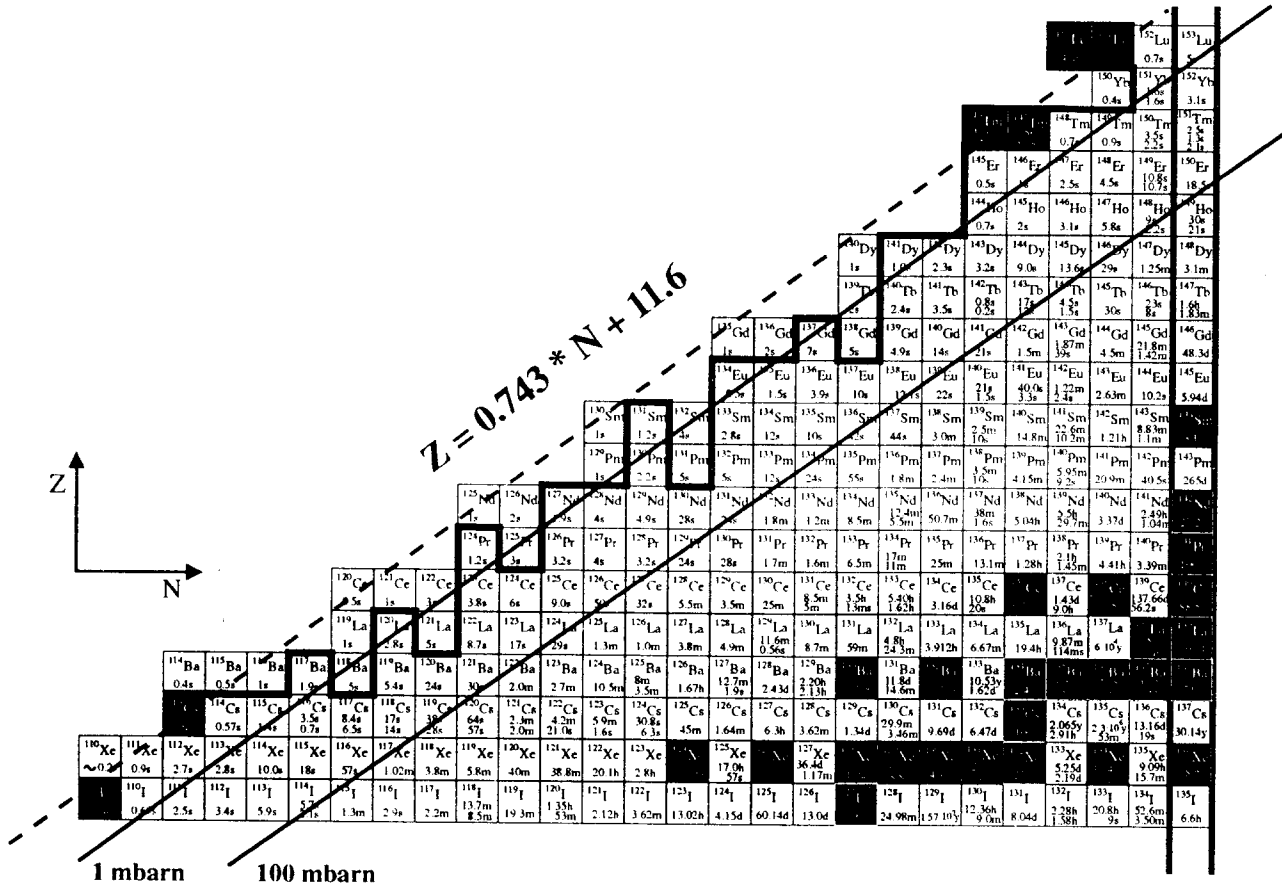
Figure 7 : Partial chart of nuclei along the proton drip line from ^{109}\text{I} to ^{151}\text{Lu} .
