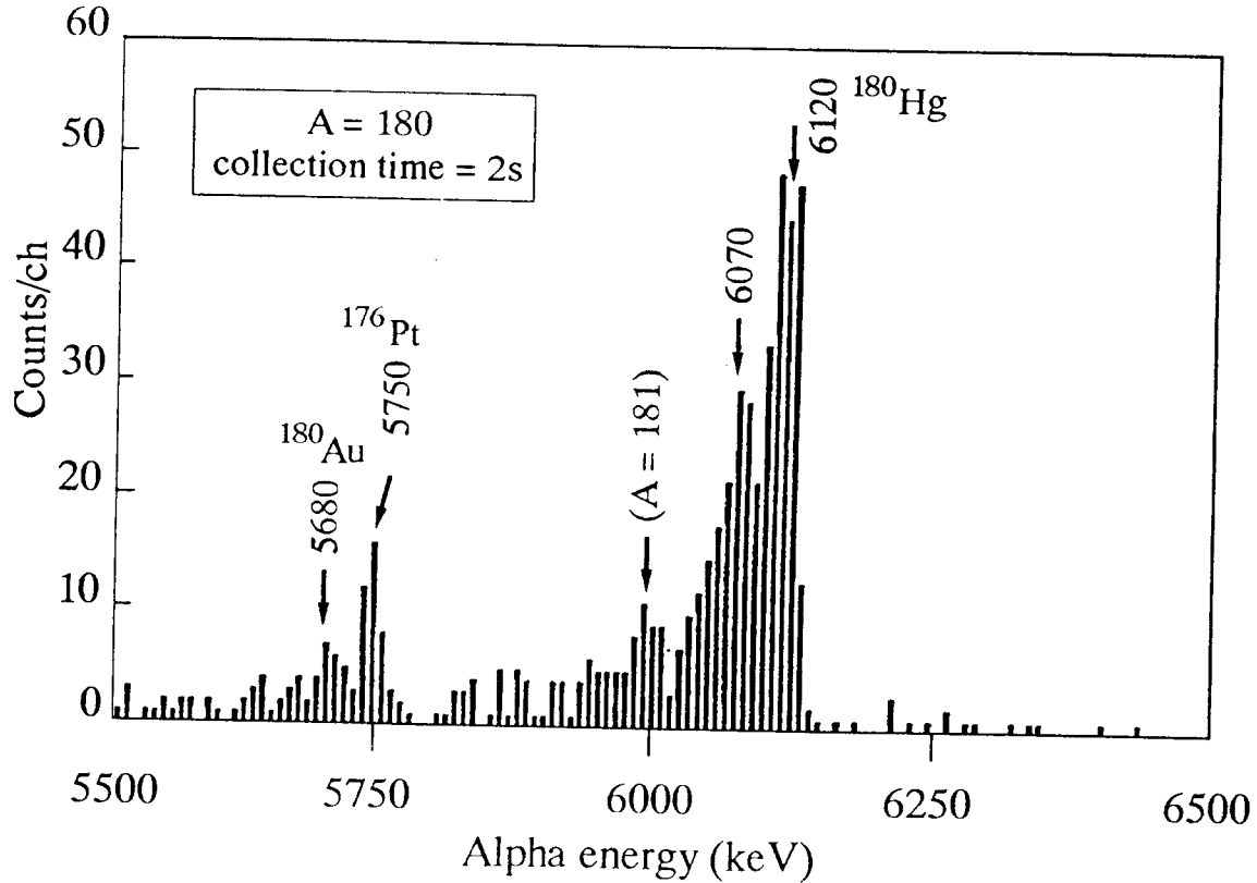
Figure 4 : \alpha -particle spectrum measured at mass A=180 for the reaction ^{144}\text{Sm} + ^{40}\text{Ca} . Collection and counting time intervals were equal to 2 seconds.
