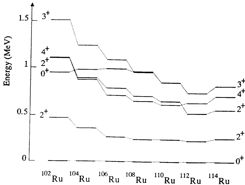
Figure 2 : Some low-lying levels of ^{102-114}\text{Ru} isotopes.
