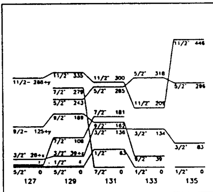
The systematics presented in Figure 6 exhibits the low-energy levels assigned via our measurement in odd-A n-deficient Ce isotopes.
