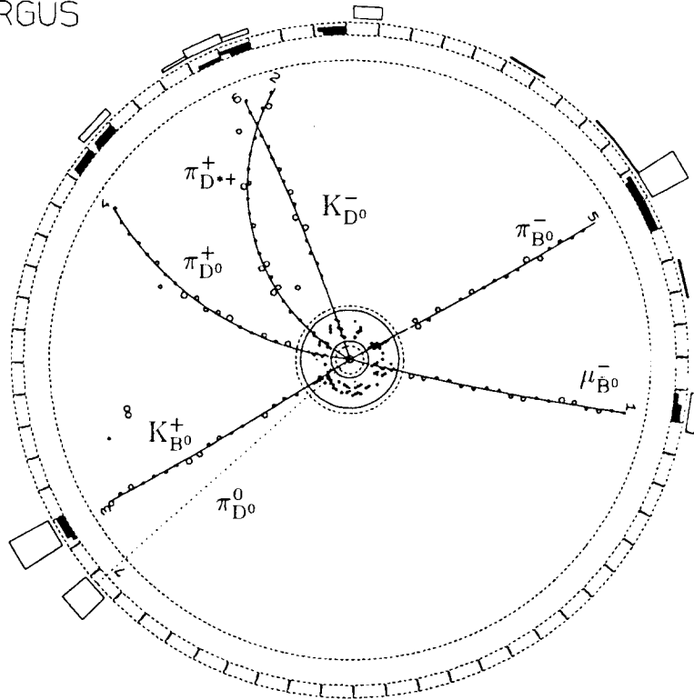
Figure 2: The completely reconstructed event with a B^0 \rightarrow K^+\pi^- candidate
