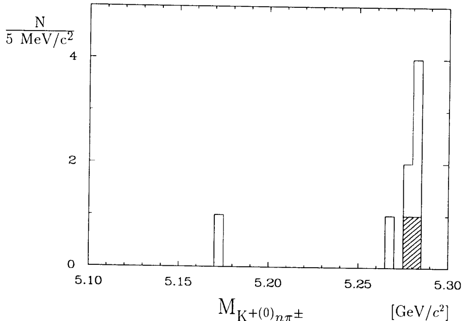
Figure 1: Invariant mass distribution for K^{+(0)}n\pi^{\pm} combinations. The hatched histogram corresponds to b \rightarrow s gluon candidates.
