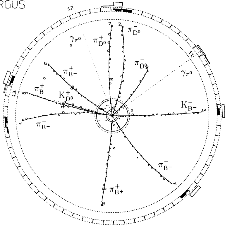
Figure 3: The completely reconstructed event with a B^- \rightarrow K^- 4\pi^\pm candidate.
