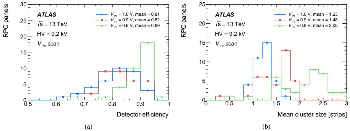
Figure 42: Distributions of (a) the panel efficiencies and (b) the mean cluster size measured at different V_{\text{thr}} threshold values with the operating voltage set to 9.2 kV.
