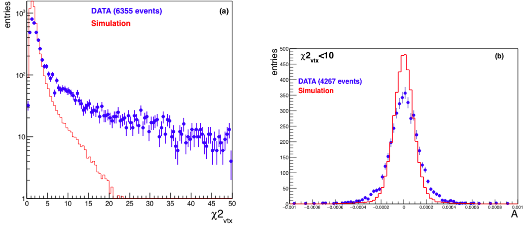
Figure 6. (a): \chi^2_{\text{vtx}} distribution. (b): acoplanarity distribution. Data are in blue with error bars, the simulated and reconstructed elastic events are the red histogram and are normalized to the observed number of events in data.
