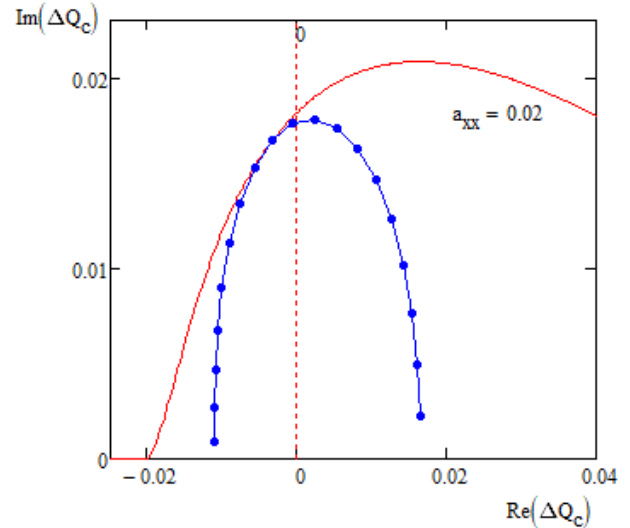
Figure 9: Stability diagram computed with accounting noise driven diffusion (blue curve) and without it (red curve.)
