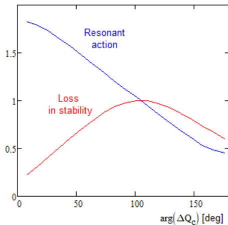
Figure 10: Dependence of the resonant action and the loss in stability on the angle of the coherent tune shift in the complex plane.
