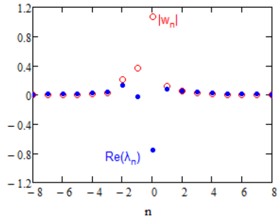
Figure 6: Dependencies on the head-tail mode number for |\hat{w}_n| (red circles) and the damping rate (blue dots).
