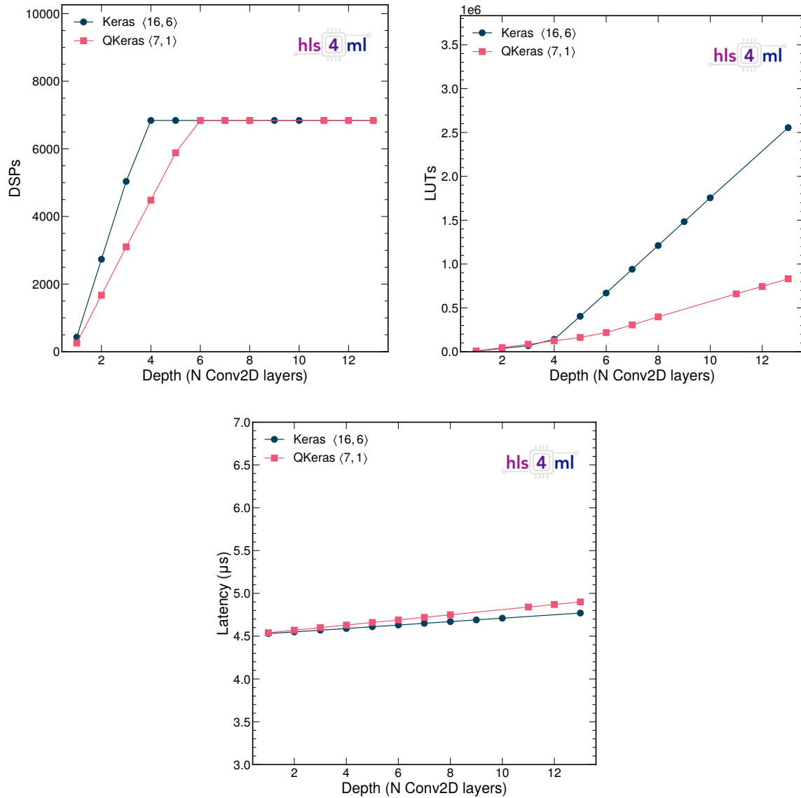
Figure 18: The DSP usage (top left), LUT usage (top right) and latency (bottom) as a function of the model depth for models using a precision of \langle 16, 6 \rangle and \langle 7, 1 \rangle . An input size of (30 \times 30 \times 3) is always assumed and each convolutional layer consists of 16 filters and a kernel size of (3 \times 3) .
