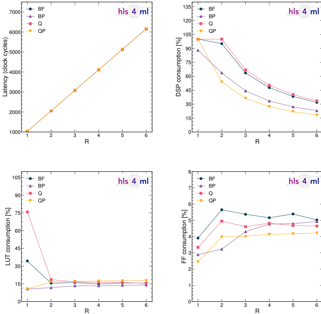
Figure 16: The model latency (top left), DSP (top right), LUT (bottom left) and FF (bottom right) consumption as a function of reuse factor for a fixed bit width of 16 for the Baseline (BF), Baseline Pruned (BP), QKeras (Q), and QKeras Pruned (QP) models.
