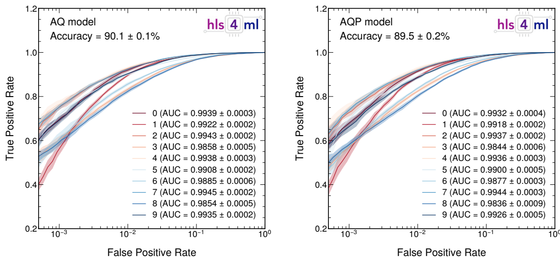
Figure 9: ROC curves of false positive rate (FPR) versus true positive rate (TPR) for the AutoQ (AQ) model (left) and the AutoQ Pruned (AQP) model (right). Training is performed using k -fold cross validation, with k = 10 . For each digit, the solid line corresponds to the mean across the ten folds and the band to the standard deviation. The mean area under the curve (AUC) across the ten folds is reported in the legend. The mean accuracy and its standard deviation across the ten folds is reported as well.
