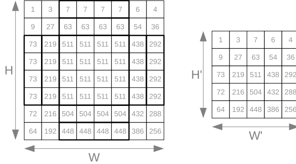
Figure 2: Example of compression of the instruction array. The left image shows the binary mask corresponding to each pixel, here represented as an integer rather than as a bit sequence. The shown values are specific of a 3 \times 3 kernel with unit stride. Instruction duplicates are highlighted by the bold-line rectangles. On the right image, we reduce the instruction array by computing the instruction array of a 5 \times 5 image, which has no duplicates, and translating the position of the element in the input array to the compressed array.
