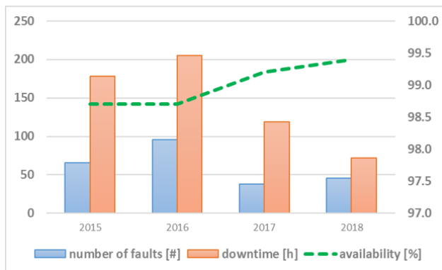
Figure 2: Run 2 overall number of faults, downtime and availability.
