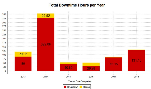
Figure 9: Lifts total downtime and origin of failure.
