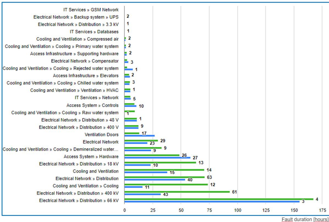
Figure 4: Pareto of all Technical Infrastructure Systems plotting the total, root causes and inherent systems downtime.
