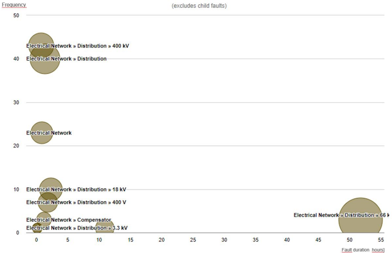
Figure 6: Electrical sub-systems downtime contribution and frequency of failures.
