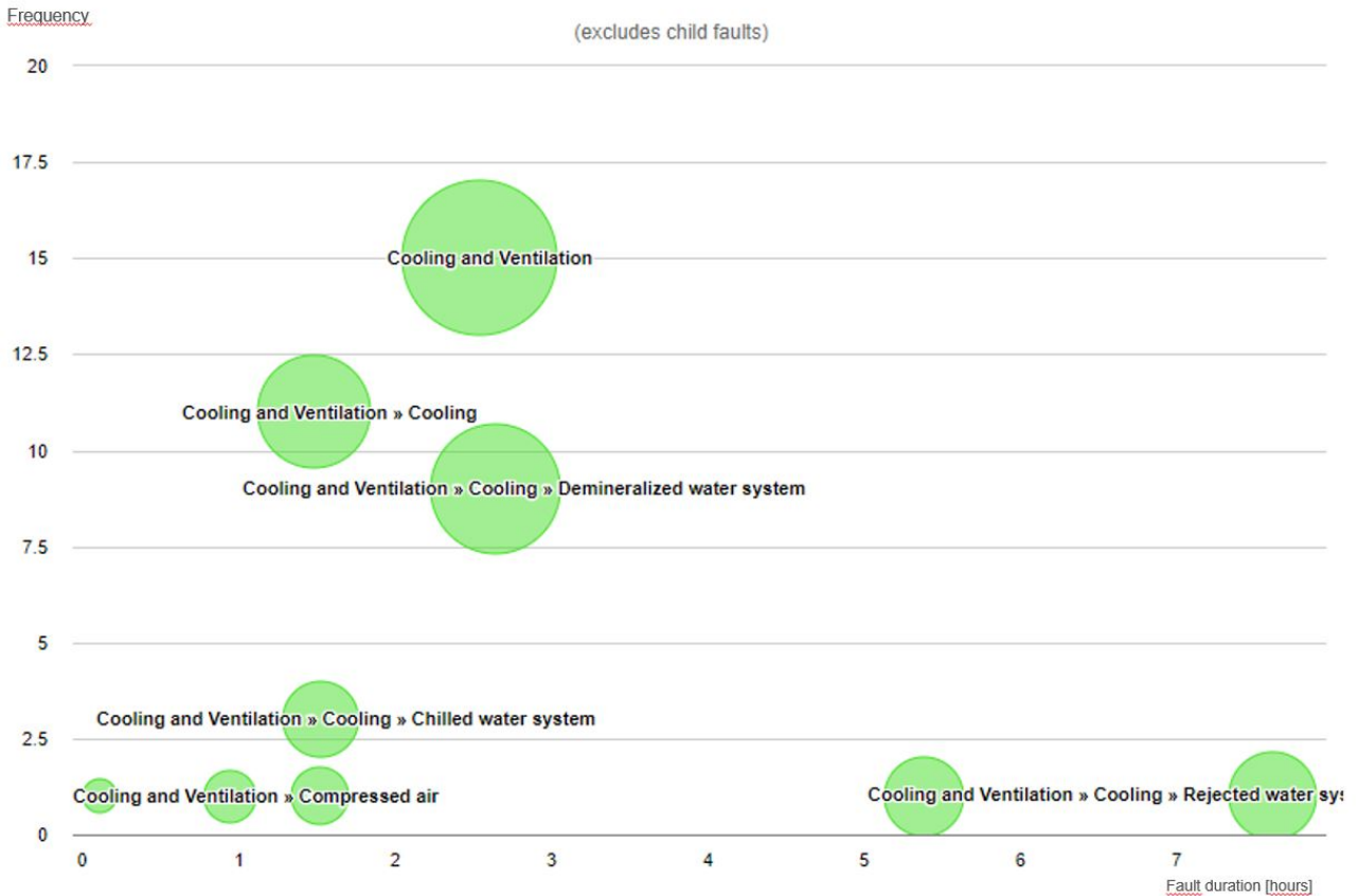
Figure 8: Cooling and Ventilation Sub-Systems downtime contribution and frequency of failures.
