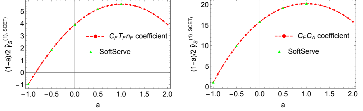
Figure 6. Soft anomalous dimension for angularities (multiplied by (1-a)/2 ) corresponding to the parameter a : coefficient of T_F C_F n_F (left) and C_A C_F (right) color factors.
