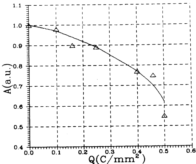
Fig.10. The dependence of the anode signal amplitude on the total collection of local charge. Anode voltage is 2.2 kV. Resistive straw: 70 kOhm/sq,
