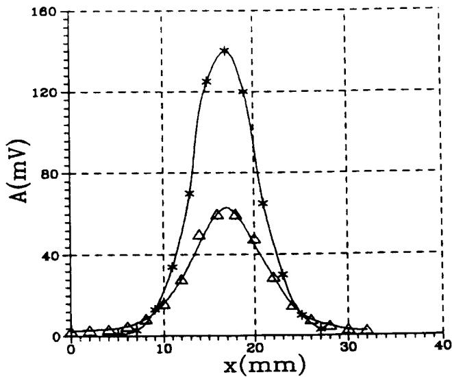
Fig. 6. The distribution of cathode signals of X-ray source position along the 10 mm diameter straw. (*) — single straw; (Δ) — 44 straws. (a), (b) — cathode resistivity 30 and 70 kOhm/sq, respectively
