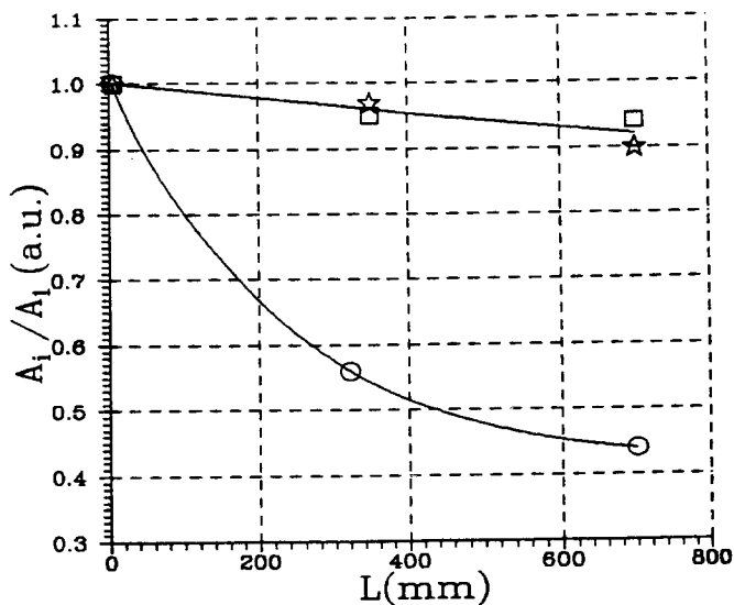
Fig. 3. The distribution of cathode signals of X-ray source position along the strip bus. (O) — 4 mm capton straws; (*, □) — 30 and 70 kOhm/sq, 10 mm diameter resistive straws
