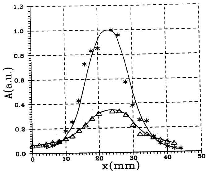
Fig. 4. The distribution of cathode signals of X-ray source position along the capton resistive stripped straw. (*) — single straw; (Δ) — 15 straws
