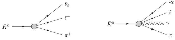
Figure 1: Radiative corrections to semileptonic K_{\ell 3} decays at O(\alpha_{\text{em}}) require the evaluation of the rates for both the processes K \rightarrow \pi \ell \bar{\nu}_\ell and K \rightarrow \pi \ell \bar{\nu}_\ell \gamma ; the corresponding amplitudes are sketched schematically here.
