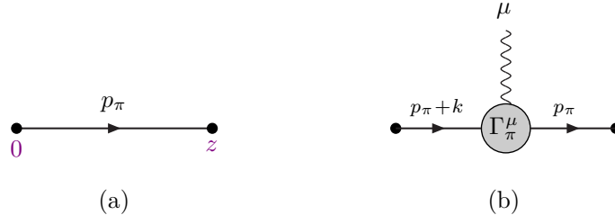
Figure 4: (a) The pion propagator, (b) \pi\gamma\pi vertex
