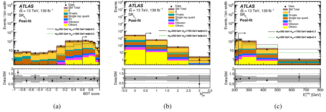
Figure 12: Representative distributions of (a) BDT score, (b) N_{\text{jet}}^{\text{forward}} and (c) E_{\text{T}}^{\text{miss}} in the t_{\text{J1L}} channel. Observed data are compared with post-fit SM predictions. All SR selections except the one on the quantity shown are applied. The SR requirement is indicated by the arrow. The ‘Others’ category includes contributions from Z +jets and tWZ production, and rare processes such as triboson, t\bar{t}t\bar{t} , t\bar{t}WW , and Higgs boson production processes. The expected distributions for representative scenarios with different m_a , m_{H^\pm} , and \tan\beta are shown for illustrative purposes. The overflow events, where present, are included in the last bin. The lower panels show the ratio of data to the background prediction. The hatched error bands indicate the combined experimental and MC statistical uncertainties on these background predictions.
