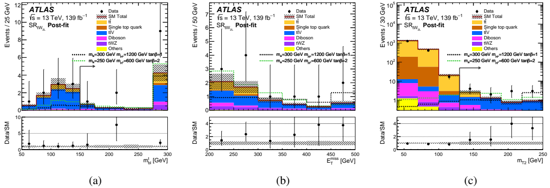
Figure 11: Representative distributions of (a) m_{b\ell}^t , (b) E_T^{\text{miss}} and (c) m_{T2} in the tW_{2L} channel. Observed data are compared with post-fit SM predictions. All SR selections except the one on the quantity shown are applied. The SR requirement is indicated by the arrow. As the m_{b\ell}^t is defined for events with at least two jets, the events with exactly one jet are included in the overflow bin. The ‘Others’ category includes contributions from rare processes such as triboson, t\bar{t}\bar{t} , t\bar{t}WW , and Higgs boson production processes. The expected distributions for representative scenarios with different m_a , m_{H^\pm} , and \tan\beta are shown for illustrative purposes. The overflow events, where present, are included in the last bin. The lower panels show the ratio of data to the background prediction. The hatched error bands indicate the combined experimental and MC statistical uncertainties on these background predictions.
