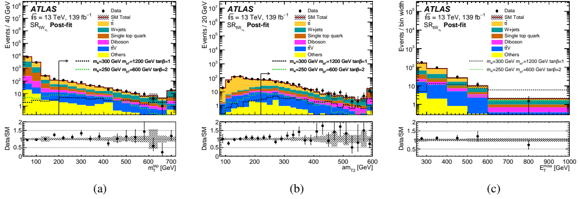
Figure 10: Representative distributions of (a) m_T^{\text{lep}} , (b) am_{T2} and (c) E_T^{\text{miss}} in the tW_{\text{IL}} channel. Observed data are compared with post-fit SM predictions. All SR selections except the one on the quantity shown are applied. The SR requirement is indicated by the arrow. The ‘Others’ category includes contributions from Z +jets and tWZ production, and rare processes such as triboson, t\bar{t}\bar{t} , t\bar{t}WW , and Higgs boson production processes. The expected distributions for representative scenarios with different m_a , m_{H^\pm} , and \tan\beta are shown for illustrative purposes. The overflow events, where present, are included in the last bin. The lower panels show the ratio of data to the background prediction. The hatched error bands indicate the combined experimental and MC statistical uncertainties on these background predictions.
