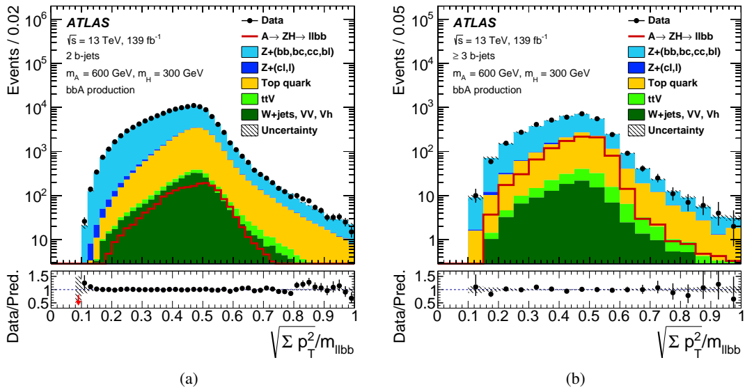
Figure 2: The \sqrt{\sum p_T^2}/m_{\ell\ell bb} distributions shown before the requirement on this variable is applied for events with (a) exactly two b -jets and (b) three or more b -jets. Corrections from a fit to the data are applied to the simulation, as described in Sections 5.1 and 8. The signal distribution for (m_A, m_H) = (600, 300) GeV is also shown, and is normalised such that the production cross section times the branching ratios B(A \rightarrow ZH) and B(H \rightarrow bb) corresponds to 1 pb. The signal shown includes only A bosons produced in association with b -quarks. The lower panel shows the ratio of the data to the background prediction (black filled circles) and the relative uncertainty, which includes both statistical and systematic components, in the background prediction (hatched area). The notations ttV , VV and Vh refer to top-pair production in association with a vector boson, diboson production and SM Higgs boson production in association with a vector boson, respectively. The production of a Z boson in association with jets is split based on jet flavour. The notation Z+(bb, bc, cc, bl) refers to the case where the jets originate from heavy flavour, which includes at least one jet originating from a b -quark or two jets originating from c -quarks, whereas the notation Z+(cl, l) includes all the remaining cases.
