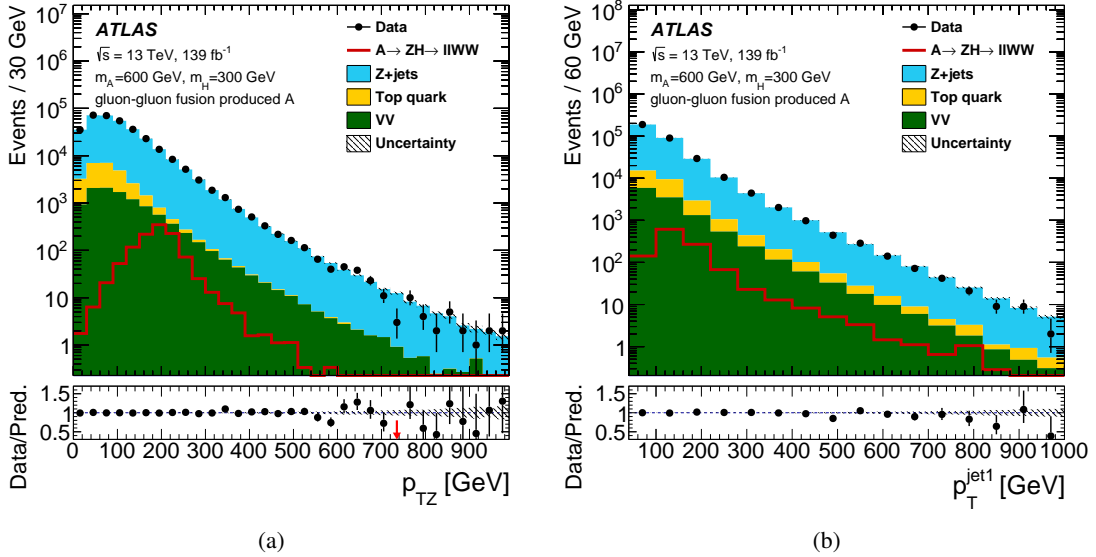
Figure 5: The distributions of (a) the p_T of the Z boson candidates and (b) the leading jet's p_T in the \ell\ell WW channel. The events are required to satisfy all the signal region criteria with the exception of the m_{4q} window requirement. Data-driven corrections are applied, as described in the text. The same conventions as in Figure 4 are used.
