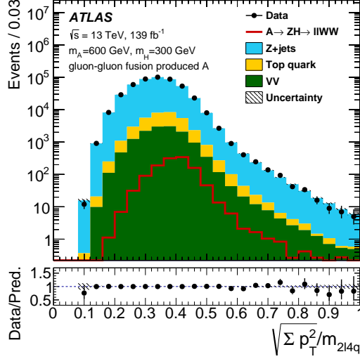
Figure 4: The \sqrt{\Sigma p_T^2}/m_{2\ell 4q} distribution shown before the requirement on this variable is applied. Corrections from a fit to the data are applied to the simulation, as described in Sections 5.2 and 8. The notation VV in the legend corresponds to the production of diboson events. The signal distribution for (m_A, m_H) = (600, 300) GeV is also shown, and is normalised such that the production cross section times the branching ratios B(A \rightarrow ZH) and B(H \rightarrow WW) corresponds to 1 pb. The lower panel shows the ratio of the data to the background prediction (black filled circles) and the relative uncertainty, which includes both statistical and systematic components, in the background prediction (dashed area).
