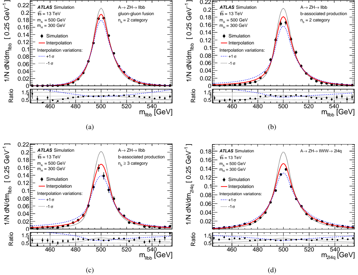
Figure 6: Signal m_{llbb} or m_{2l4q} distributions assuming m_A = 500 GeV and m_H = 300 GeV for the following cases: llbb channel: (a) gluon-gluon fusion in the n_b = 2 category, (b) b -associated production in the n_b = 2 category, and (c) b -associated production in the n_b \geq 3 category; (d) llWW channel. In the upper panels, the black filled circles correspond to the simulated distributions, which are compared against the interpolated parameterised signal distributions shown as solid red curves. Also in the same panels, the shape variations of the interpolated parameterised signal distributions are shown in dotted blue ( +1\sigma ) and black ( -1\sigma ) lines. In the lower panels, the black filled circles correspond to the ratio of the simulation to the interpolated parameterised curve. The dotted blue (black) line corresponds to the ratio of the +1\sigma ( -1\sigma ) shape variation of the interpolated curve to the interpolated curve.
