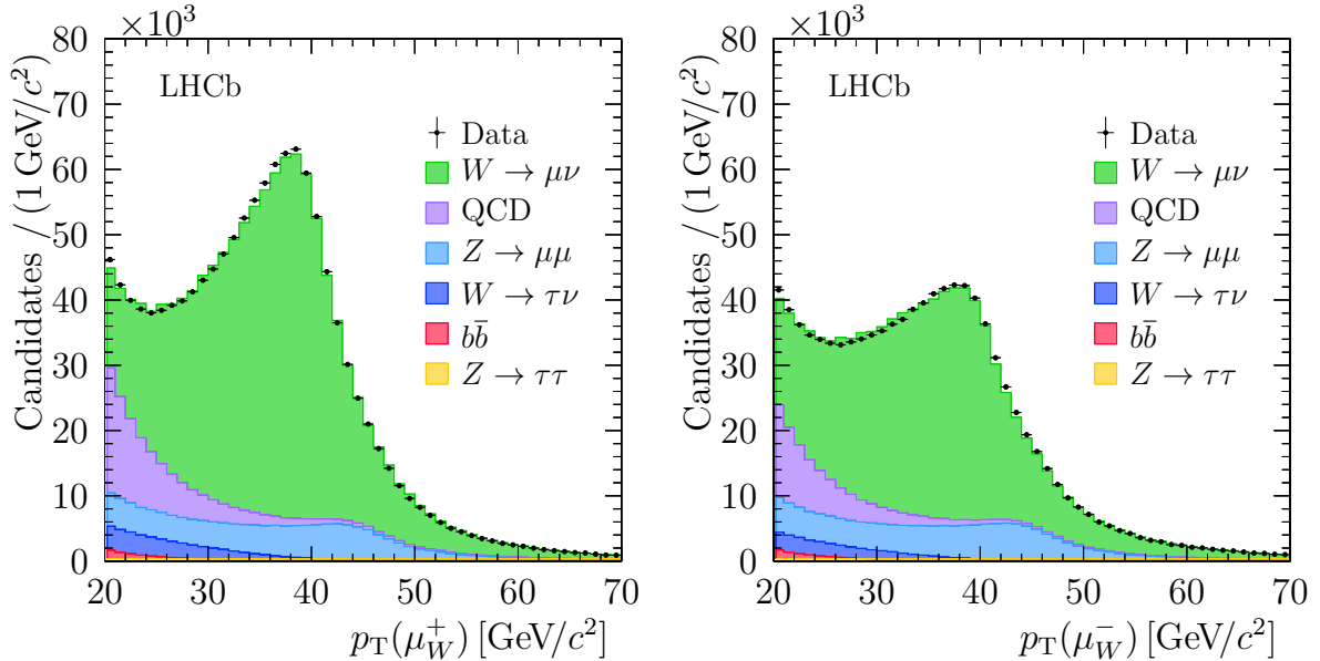
Figure 3: The (left) positive and (right) negative muon transverse momentum spectra for the 2012 data set integrated over pseudorapidity for the normalisation channel. The fit is overlaid.
