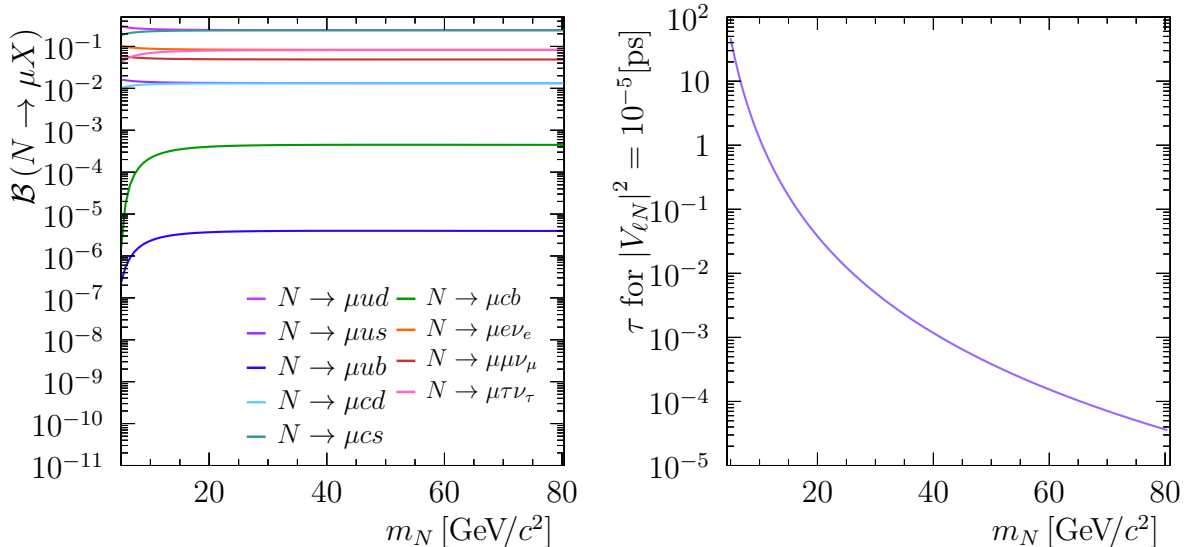
Figure 1: Properties of a heavy neutrino as a function of its mass [21, 22]: (left) the branching fractions to final states with a muon and (right) the lifetime, assuming a coupling of 10^{-5} (current limit).
