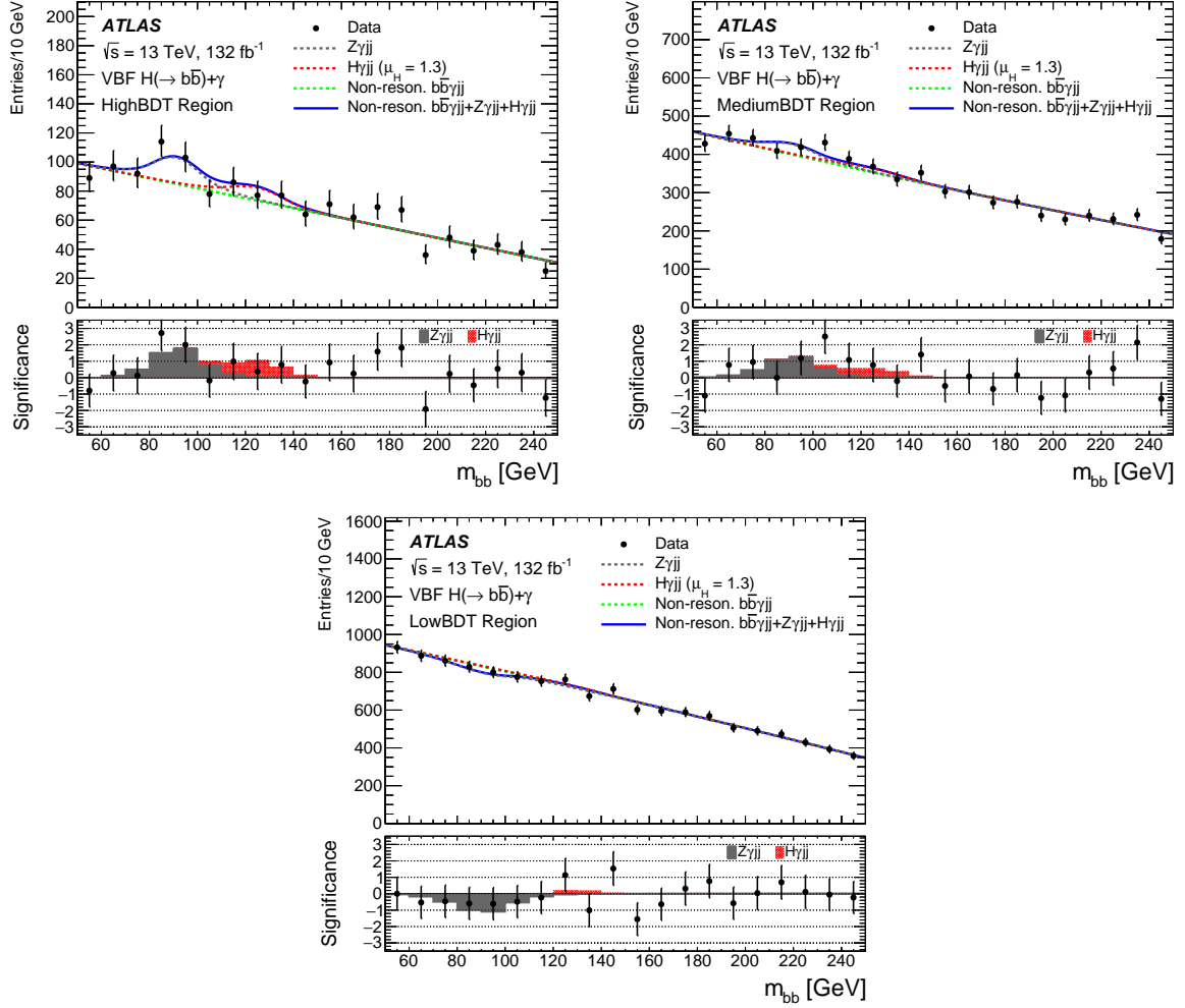
Figure 5: The m_{bb} distributions in the three event categories, overlaid with contributions from the H\gamma jj signal as well as the resonant Z\gamma jj and non-resonant bb\bar{\gamma}jj background fits. The combined \chi^2 per degree of freedom is 45.2/45. The bottom panel in each plot presents the significance of the Higgs boson signal relative to the non-resonant bb\bar{\gamma}jj background in each bin, calculated using a Poisson model [47].
