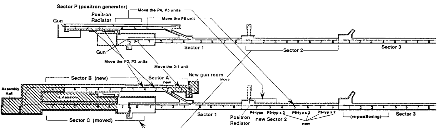
Fig.1 The linac re-formation from 2.5 GeV (upper) to 8 GeV (lower). The shadow area is an extension for expanding the linac length; accelerator units are to be increased from 40 to 57. The present positron generator is to be moved from Sector P to Sector 2; the primary electron energy is to be increased from 250 MeV to 3.7 GeV.
