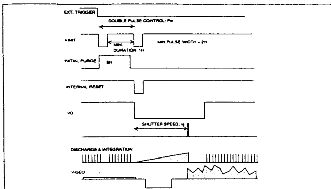
Fig. 2. Block diagram of the shutter control timing of the asynchronous-reset CCD camera.
