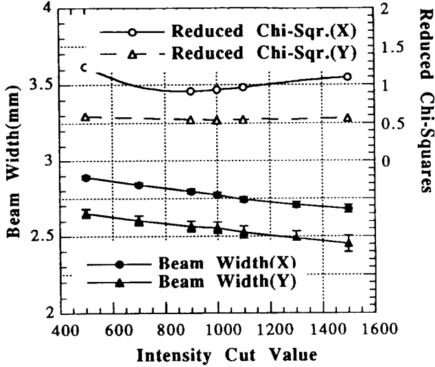
Fig. 5. Fitting characteristics by changing the intensity cut value for the beam tail. The horizontal axis is the cut value of the beam intensity and the vertical axes are the beam width ( 1\sigma ) and reduced chi-squares.
