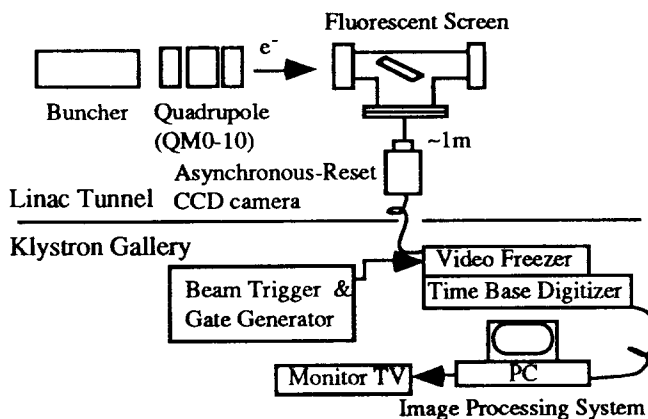
Fig. 1. Emittance measurement system at the pre-injector.
