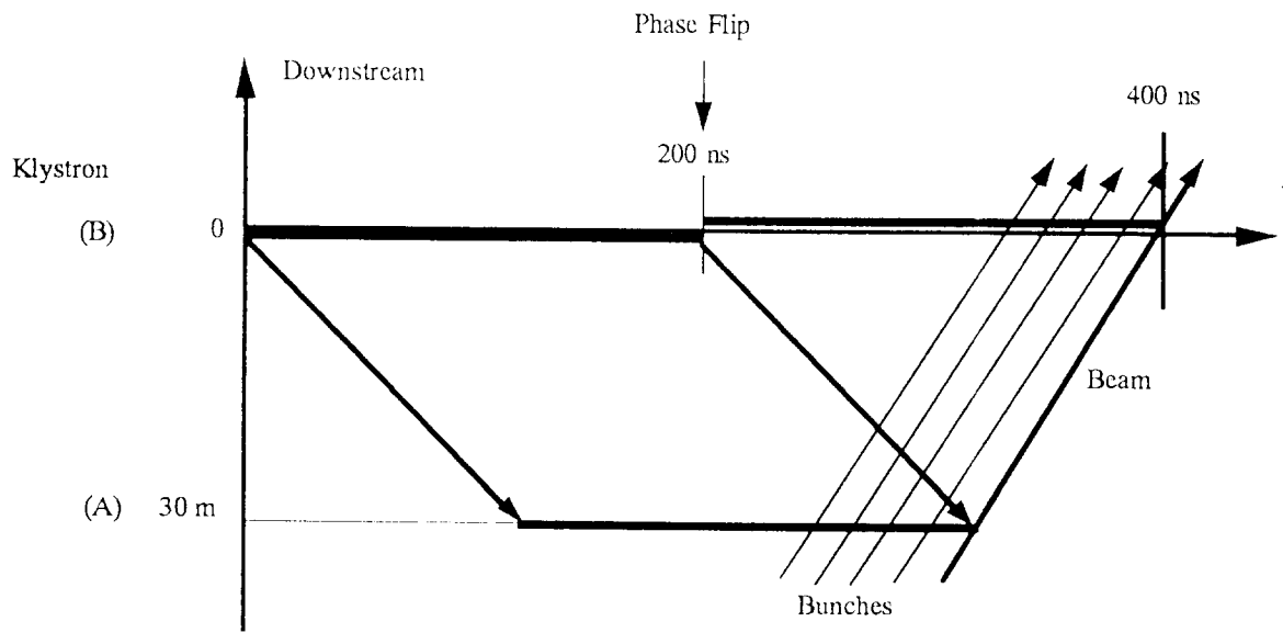
Fig-2) A railroad diagram of the delayed line distribution system
