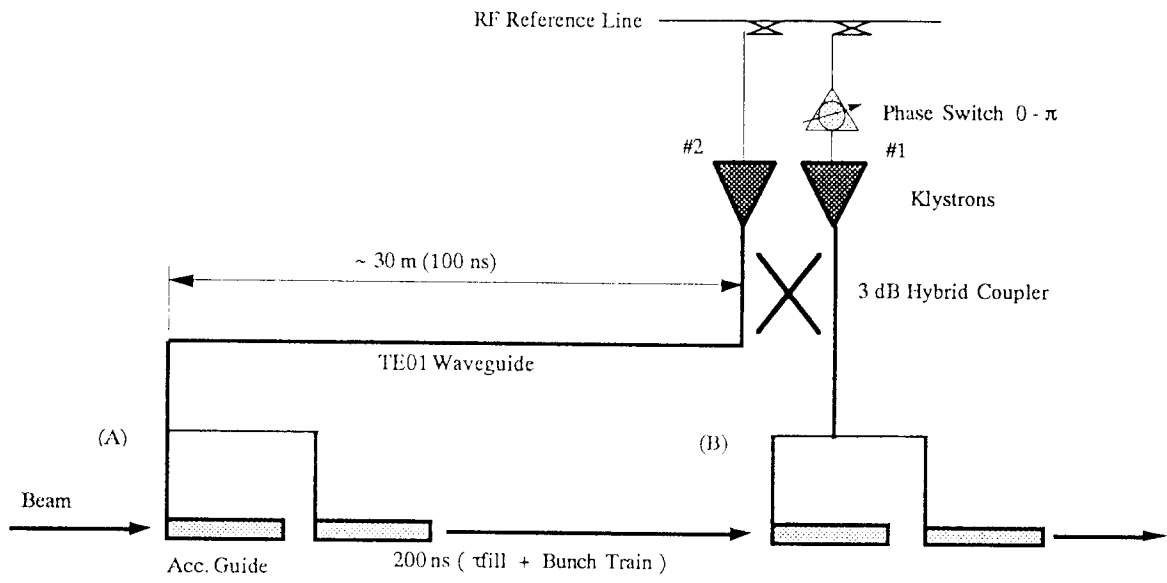
Fig-1) A schematic diagram of the delay line distribution system
