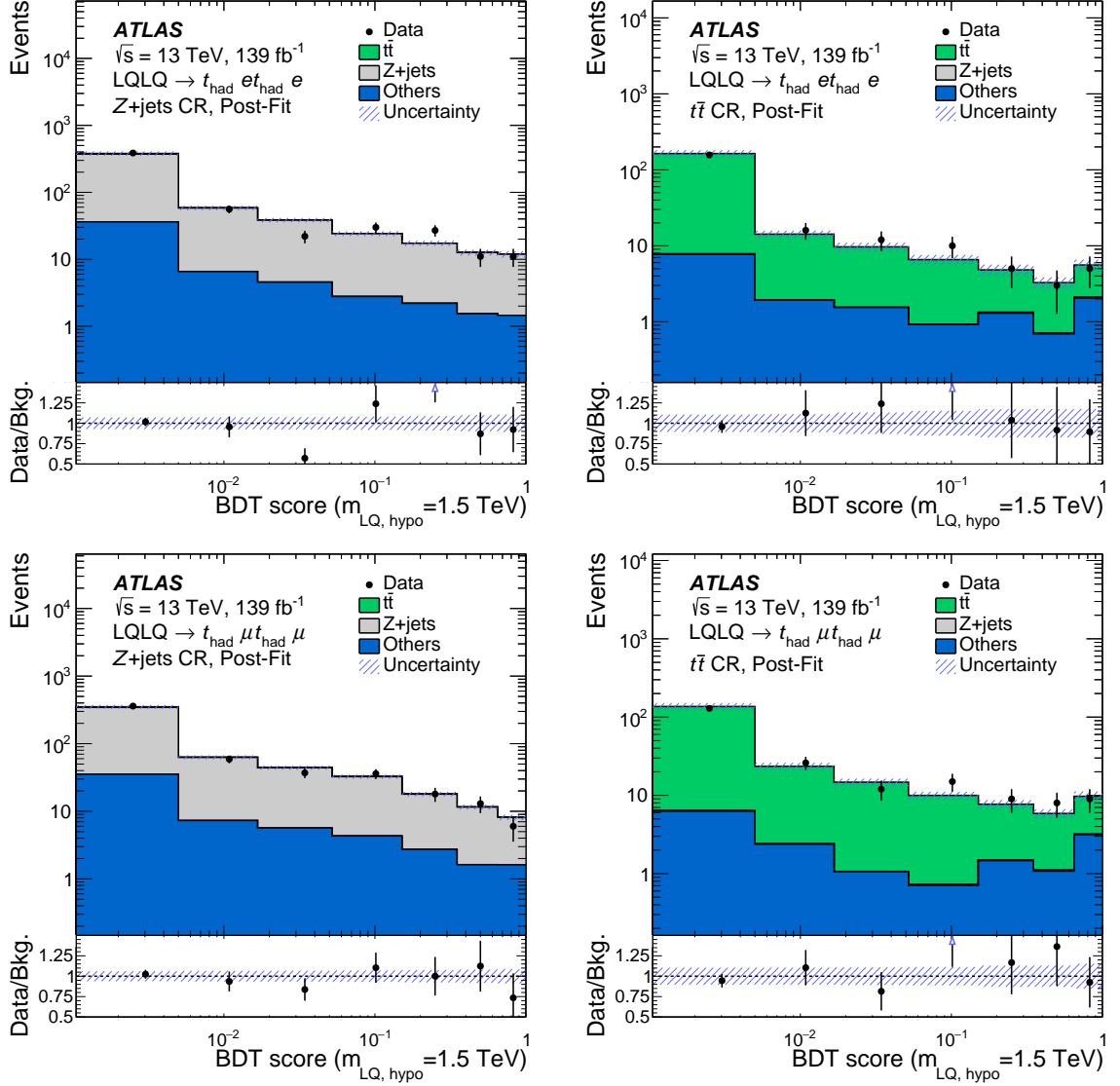
Figure 3: Distributions of the BDT output score in the Z + jets and t\bar{t} CRs for the electron (top row) and muon (bottom row) channel after the simultaneous background-only fit of the CRs. The bottom panels show the ratio of data to expected background. The hatched band represents the total uncertainty. All BDT scores correspond to the theoretical LQ mass parameter m_{LQ, \text{hypo}} set to 1.5 TeV. The first bin contains all underflow events.
