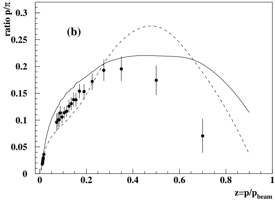
Figure 5: Ratios of the rates of (a) K^\pm/\pi^\pm and (b) (p, \bar{p})/\pi^\pm as a function of z = p_{\text{hadron}}/p_{\text{beam}} , compared with the predictions of JETSET (solid line) and HERWIG (dashed line). The errors shown are the quadratic sum of statistical and systematic errors.
