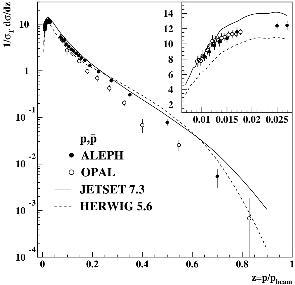
Figure 4: Differential cross-section as a function of z = p_{hadron}/p_{beam} for (p, \bar{p}) , compared with the measurement of OPAL and the predictions of JETSET and HERWIG. The errors shown are the quadratic sum of statistical and systematic errors.
