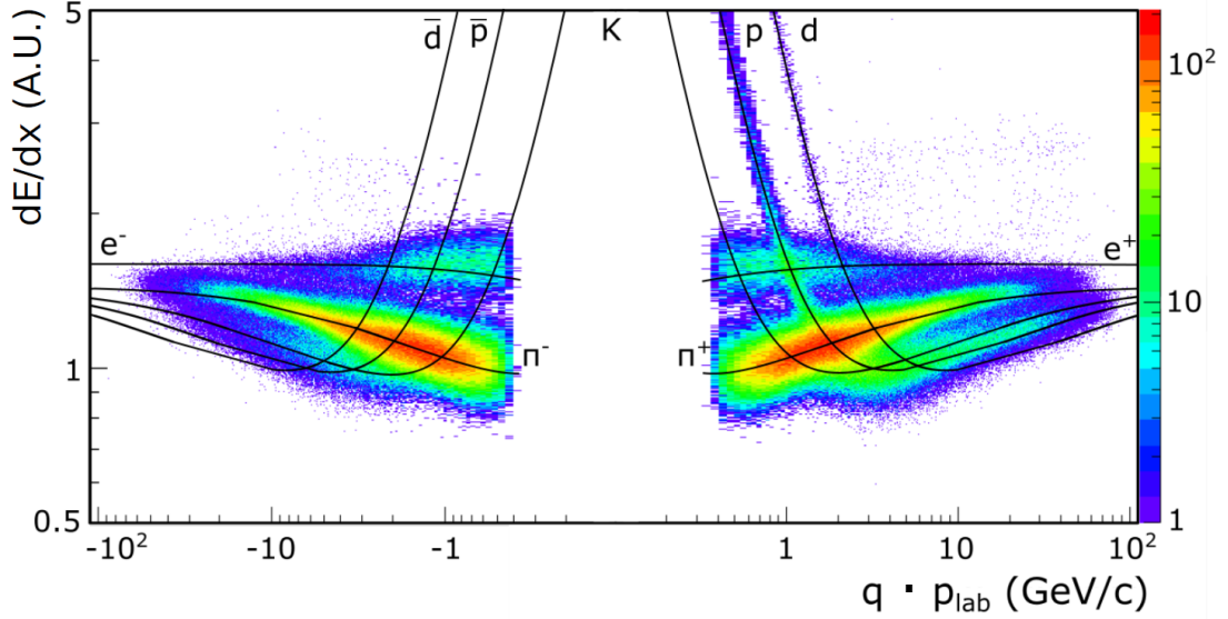
Figure 6: Acceptance of the tof-dE/dx and dE/dx methods for identification of pions, kaons and protons in the 20% most central Be+Be interactions at 150A GeV/c.
