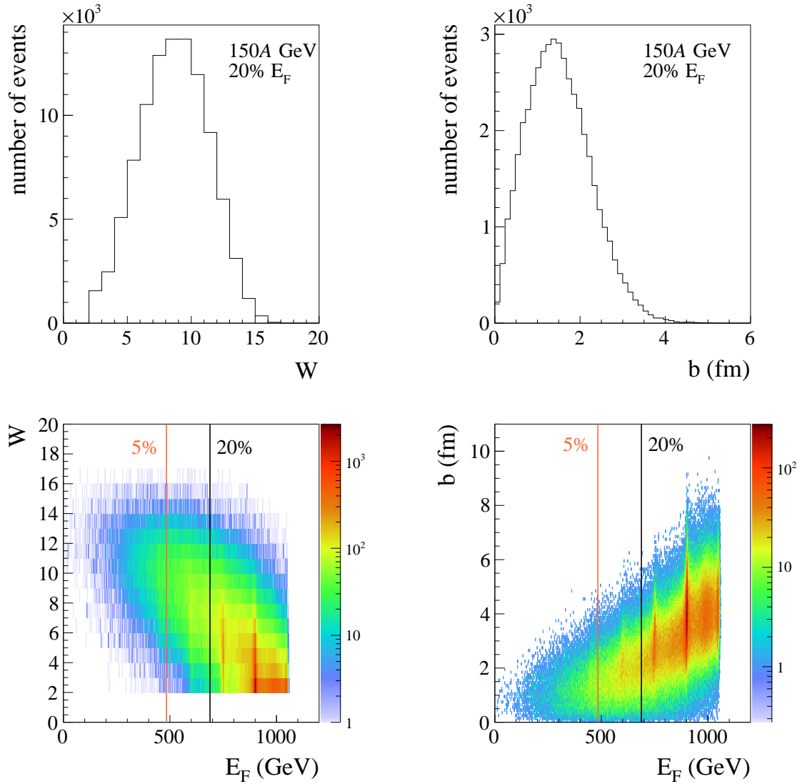
Figure 4: Examples of the distribution of the number of wounded nucleons W ( left ) and collision impact parameter b ( right ) for events with the 20% smallest forward energies E_F ( central ) at beam momentum of 150A GeV/c simulated with the EPOS model using the acceptance map provided in Ref. [18].
