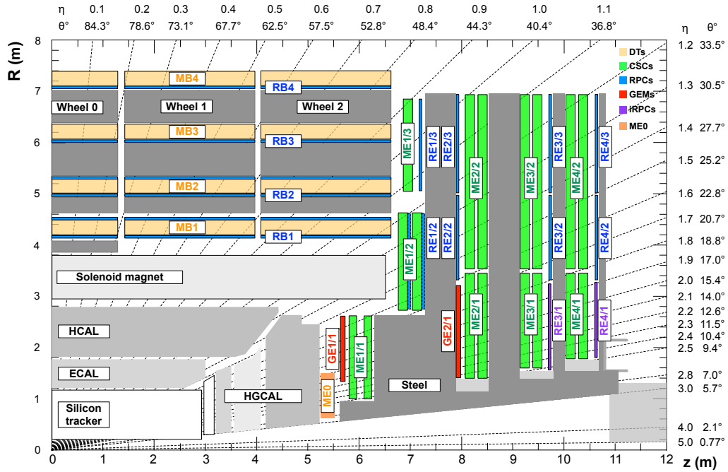
Figure 1. An R-z cross section of a quadrant of the upgraded CMS detector high-lighting the locations of the new GE1/1, GE2/1, and ME0 stations with GEM technology in the CMS muon endcap region. The previously existing muon stations, i.e. drift tubes (MB), cathode strip chambers (ME), and resistive plate chambers (RB, RE), and the flux-return steel yoke (dark areas) are also shown.
