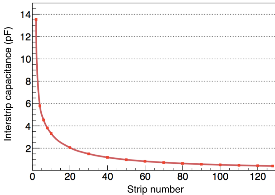
Figure 14. Interstrip capacitance between first strip and a non-adjacent strip using the multi-strip FEA model. For this calculation, a fixed potential of 1 V is applied to the first strip and a fixed potential of 0 V is applied to the other strip of interest.
