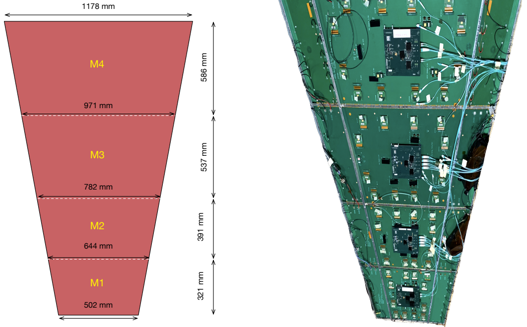
Figure 3. Left: The dimensions of the modules in the back chamber of the GE2/1 superchamber. Right: A fully instrumented GE2/1 prototype chamber.
