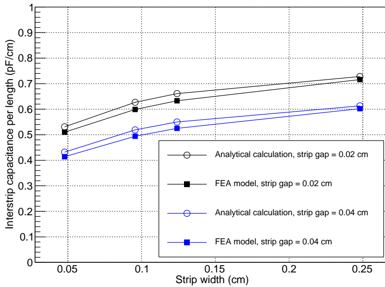
Figure 12. Comparison between analytical calculation and 2D FEA modeling of interstrip capacitances per length for original TDR strip width and doubled strip width in the M1 and M4 modules.
