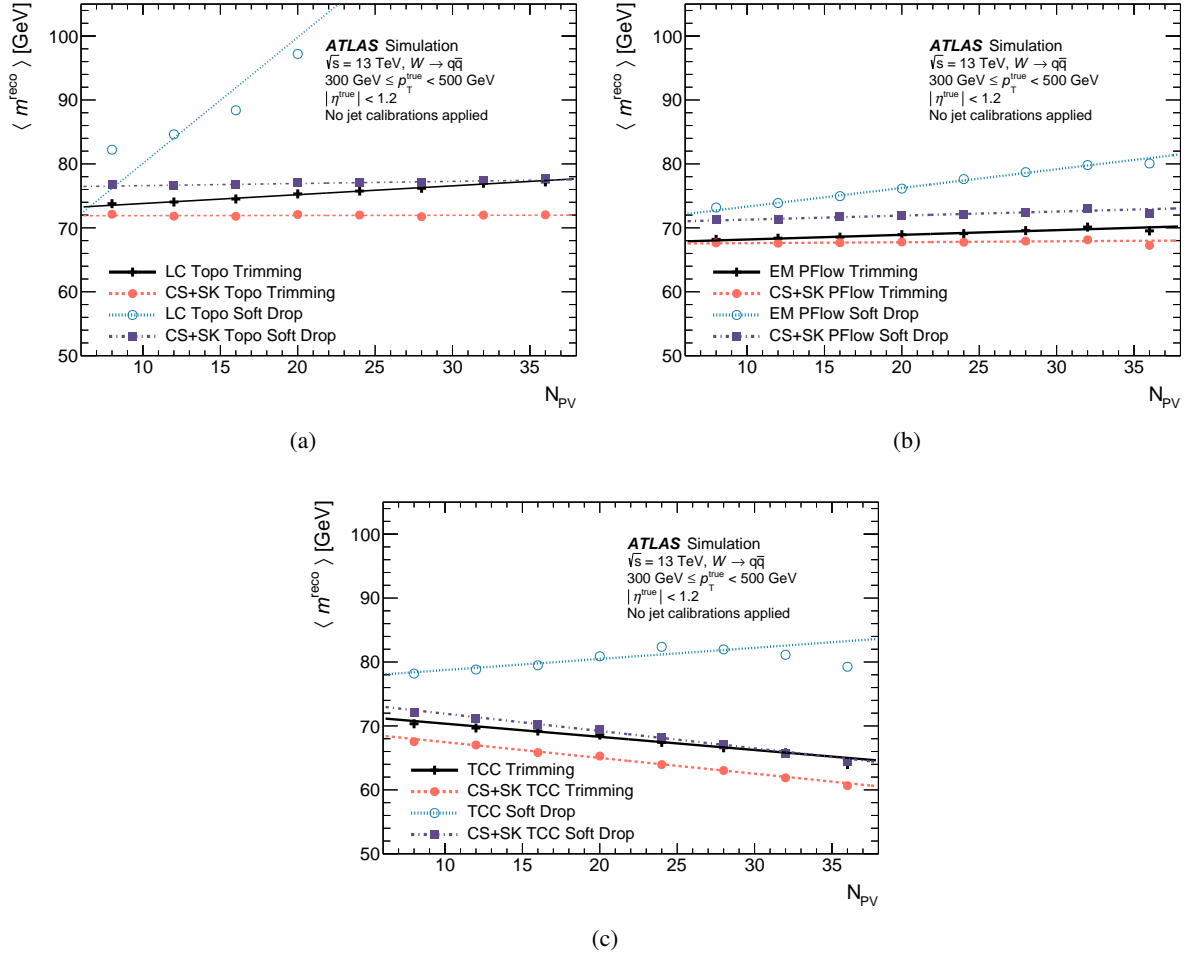
Figure 4: The value of the fitted W boson mass peak as a function of the number of primary vertices, N_{\text{PV}} . Several different jet input object types are shown: (a) topoclusters, (b) particle-flow objects and (c) track-caloclusters. Jet p_T and \eta cuts before tagging are made using the ungroomed particle-level large- R jet matched to each of the groomed reconstructed large- R jets. Jets groomed with the trimming ( R_{\text{sub}} = 0.2 , f_{\text{cut}} = 0.05 ) and soft-drop ( \beta = 1.0 , z_{\text{cut}} = 0.1 ) algorithms are shown.
