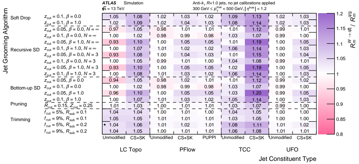
Figure 14: Ratio of the mean value of mass response in W jets to that in q/g jets at low p_T . Kinematic selections before tagging are made using the ungroomed particle-level large- R jet matched to each of the groomed reconstructed large- R jets. The current baseline topocluster-based trimmed collection is indicated with a \star .
