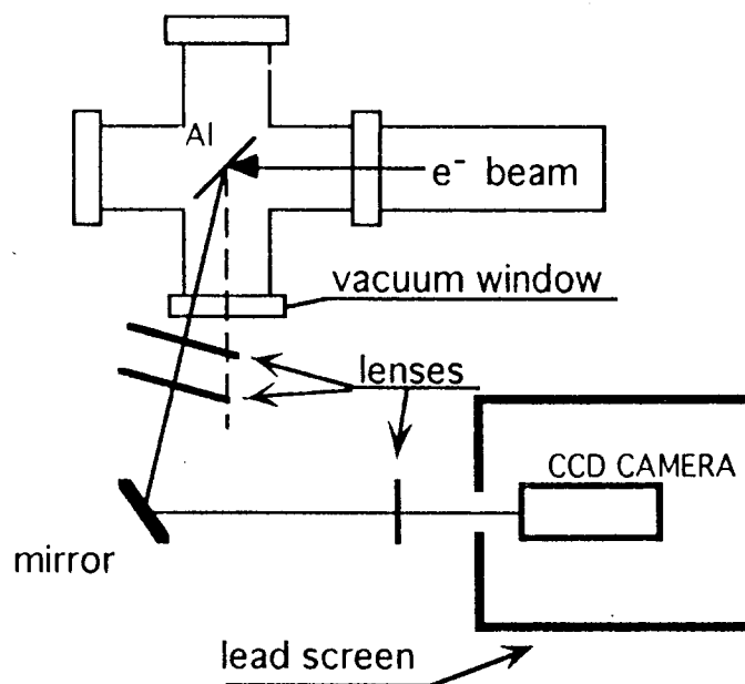
Fig. 7 - Schematic layout of the experimental set-up
