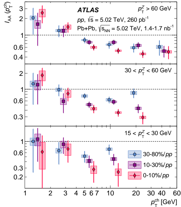
Figure 2: Ratio of the charged-particle yield in Pb+Pb collisions to that in pp collisions, I_{AA} , as a function of charged-particle p_T^{\text{ch}} . The vertical bars and boxes correspond to the statistical and systematic uncertainties of the data. The 0–10% and 30–80% data are offset horizontally for visibility.
