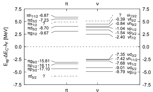
FIG. 1. Experimental single-particle and single-hole energies for neutrons ( \nu ) and protons ( \pi ) in the doubly-magic nucleus ^{132}\text{Sn} . Following [9] the energy origin is set in the center of the shell gap ( \lambda_F ) in order to remove Coulomb energy differences \Delta E_C . Binding energies are taken from [10]. The absolute single-particle energies are given in MeV.
