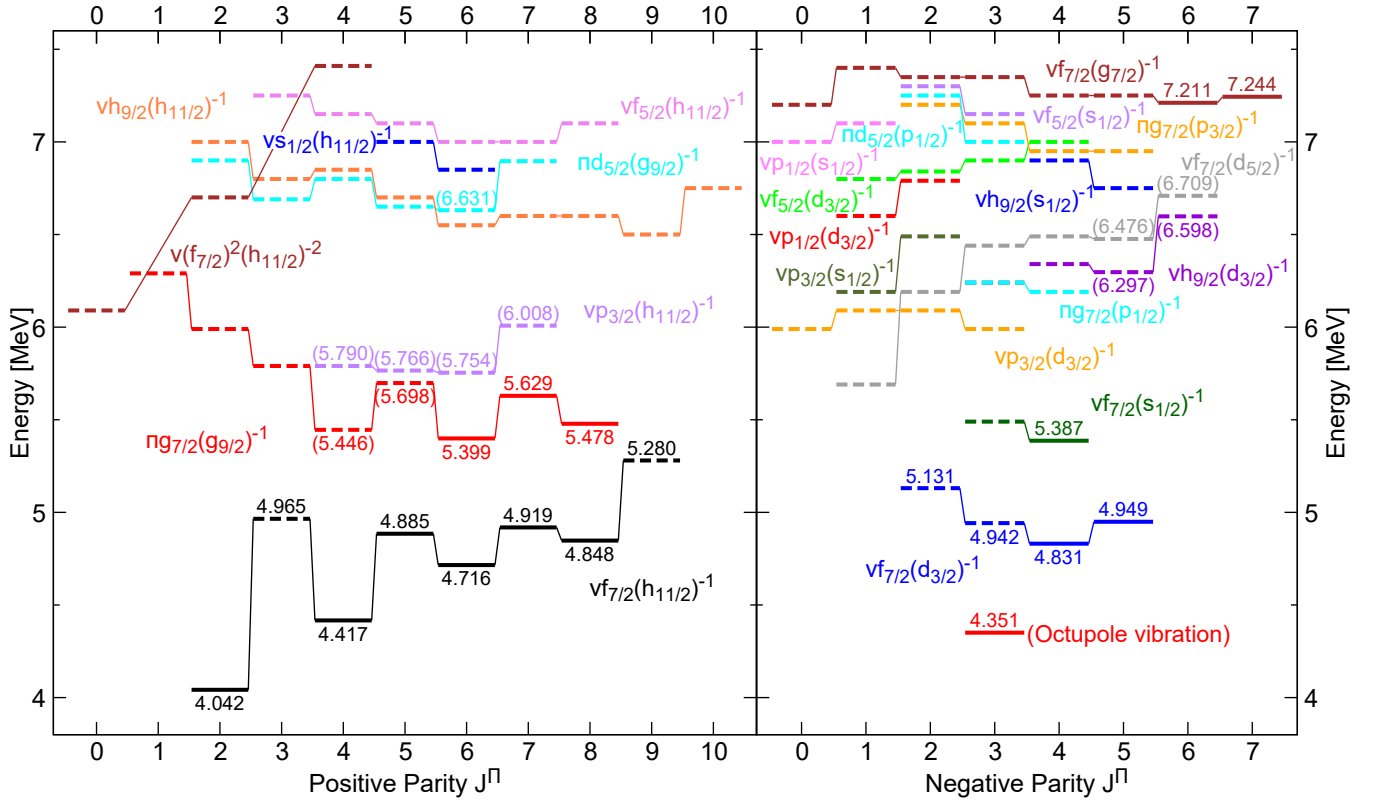
FIG. 11. Calculated energies for the different particle-hole multiplet states in ^{132}\text{Sn} , adopted from J. Blomqvist [46, 47]. The energies and energy splitting within a given multiplet are estimated by scaling the analogous particle-hole states in ^{208}\text{Pb} and taking into account single particle energies from neighboring nuclei. Previously identified levels are plotted with continuous lines. The experimental energies from our work are shown for the newly identified states. The levels whose energies appear between brackets correspond to tentative assignments.
