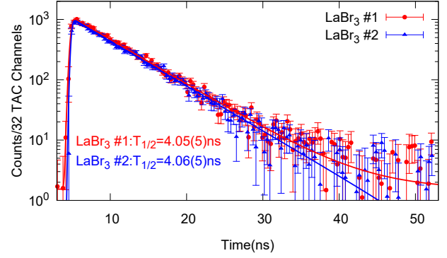
FIG. 9. Time delay spectra between the \beta and each of the two \text{LaBr}_3(\text{Ce}) detectors for \beta\gamma\gamma(t) events. These distributions are built by selecting the events when the 526-keV transition in the HPGe detectors and the 375-keV transition in the \text{LaBr}_3(\text{Ce}) detector. The lifetime is obtained by a \chi^2 fit of the whole time distribution to an exponential decay convoluted with a Gaussian function plus a constant background to account for the random background.
