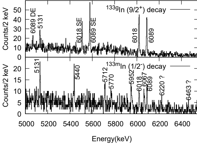
FIG. 8. Beta-gated \gamma -ray spectra from the \beta decay of ^{133}\text{In} isomers highlighting the energy range above 5 MeV. Only the events recorded in the time window from 10 to 600 ms since the arrival of the proton pulse are used.
