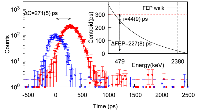
FIG. 10. Time delayed \beta\gamma\gamma(t) spectra used to measure the lifetime of the 4830-keV 4^- excited level. The blue spectra depicts the prompt time distribution used as reference, which is obtained by gating on the 479 and 2380-keV transitions in the HPGe and the \text{LaBr}_3(\text{Ce}) detectors respectively. The red one correspond to events obtained after reversing the gates, the 2380 keV one applied to the HPGe and the 479 keV one to the \text{LaBr}_3(\text{Ce}) . The shift measured between the centroid position of each distribution \Delta C is caused by the lifetime of the level, but also due to the time walk \Delta \text{FEP} between both energies. The lifetime \tau is obtained by subtracting to the centroid shift the contribution due to the FEP time response.
