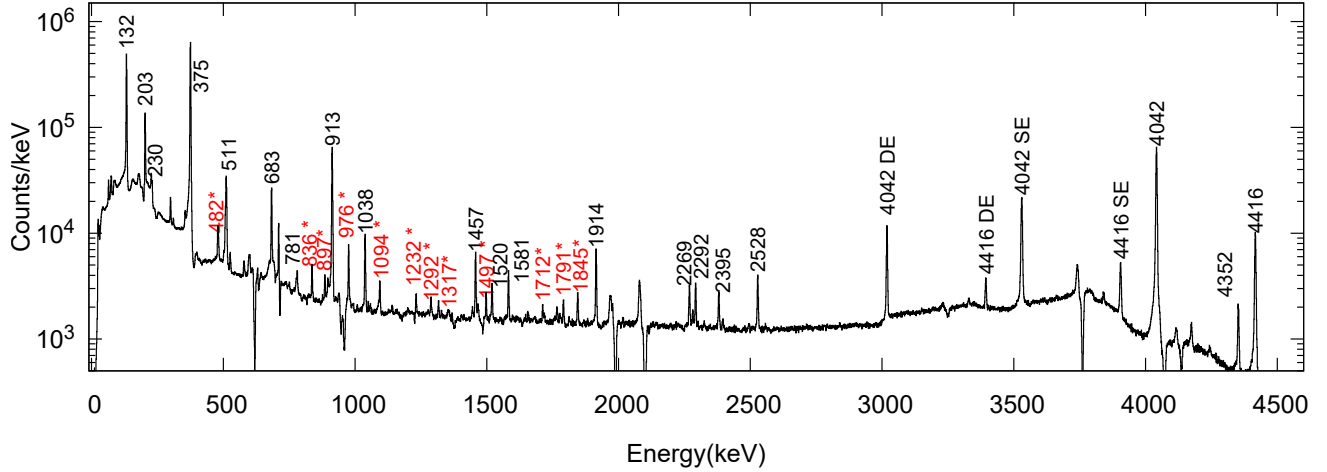
FIG. 4. Compton-subtracted \gamma - \gamma energy spectrum gated on the 6^+ \rightarrow 4^+ 299.3 keV \gamma transition in ^{132}\text{Sn} . The previously-known \gamma rays are labeled with their energies in black. New transitions identified in this work are labeled in red with an asterisk. The negative peaks in the spectrum arise from background subtraction, due to Compton scattering between two HPGe clover detectors.
