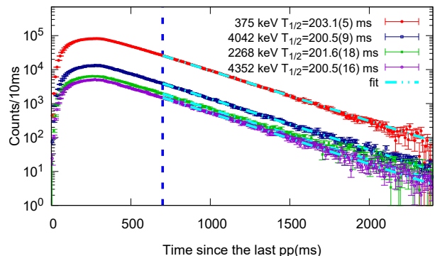
FIG. 3. Decay curves of the 375-, 4042-, 2268- and 4352-keV \gamma -rays recorded in singles in the HPGe detectors. The region considered for the fit goes from 700 ms, marked with a dark-blue dashed line, up to 2400 ms. This region has been adjusted in order to minimize dead-time effects.
