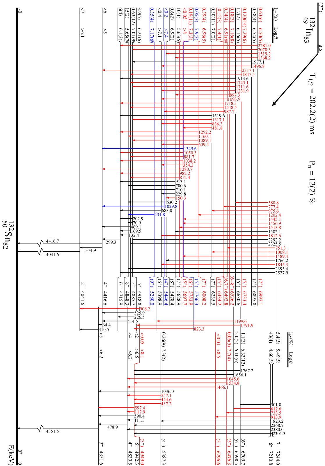
FIG. 5. Level scheme of ^{132}\text{Sn} observed following the \beta decay of ^{132}\text{In} . Note that the energy gap from the g.s. to the 2^+ state is not to scale. The positive-parity states are shown on the left-hand side and the negative parity ones on the right-hand side. The high-lying 7^- and 6^- states feed states of both parities. Levels and transitions previously observed in this decay are colored in black, while those observed for the first time are highlighted in red. Levels previously-known from ^{248}\text{Cm} fission or from ^{133}\text{In} \beta -n decay and observed here in the \beta -decay of ^{132}\text{In} are colored in blue.
