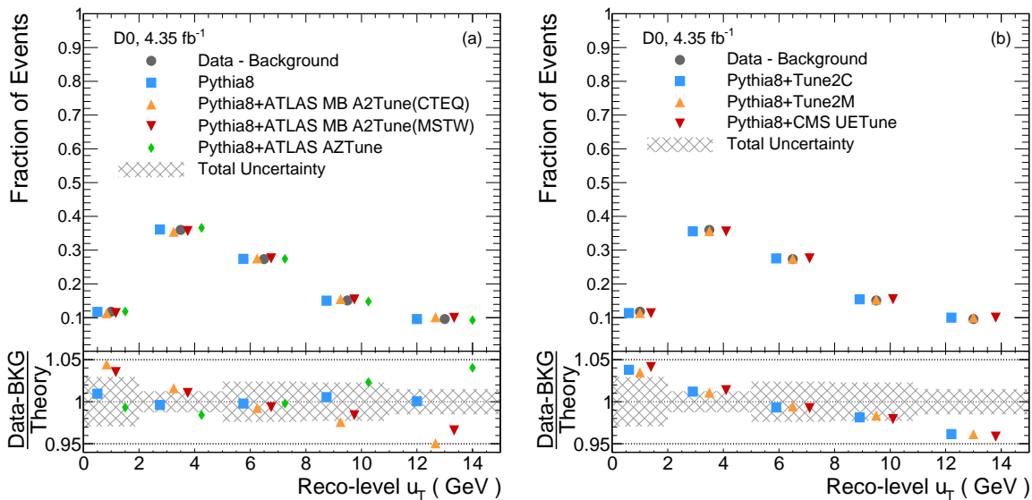
FIG. 4: [color online] Comparisons of the measured and predicted u_T distributions after the detector response simulation for different MC predictions based on PYTHIA . The ratios of the background-subtracted data to each theory prediction are shown in the lower panel together with the 1\sigma uncertainty band. The total experimental uncertainty is indicated by the hatched band; it is dominated by the uncertainty due to the hadronic recoil calibration. The points for the predictions are offset horizontally to aid with visibility.
