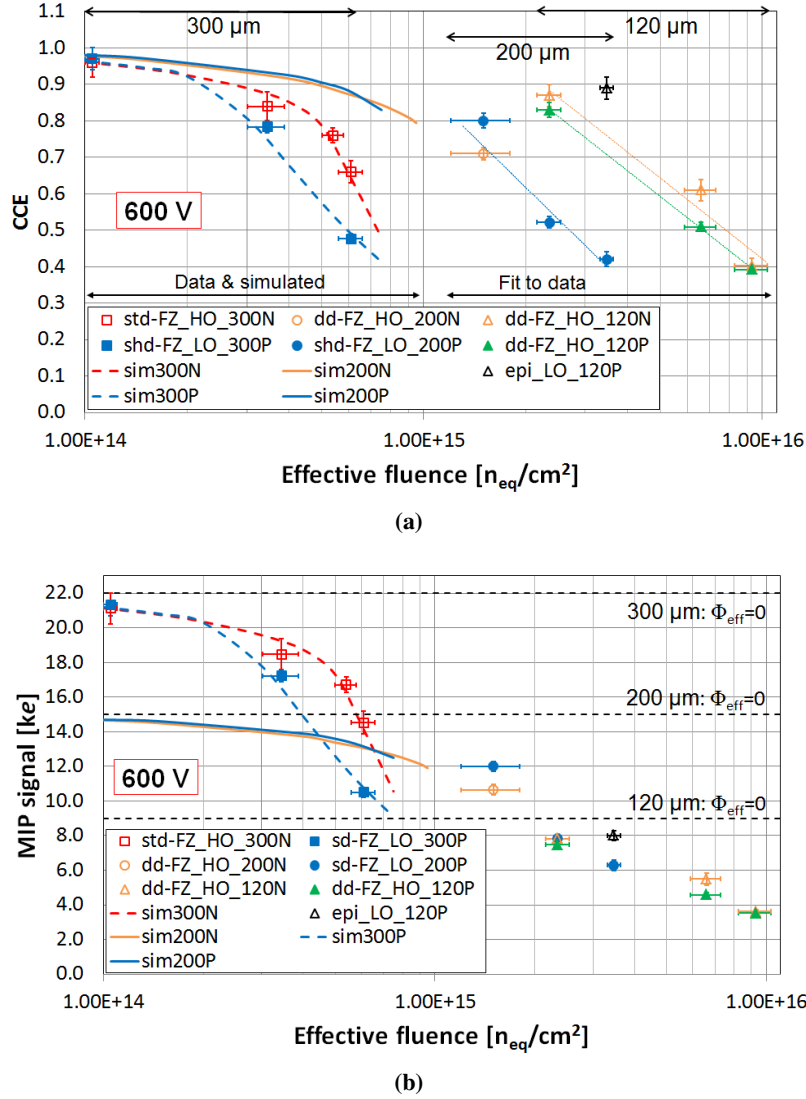
Figure 8. CCE and MIP charge collection as a function of fluence for the three sensor thicknesses at 600 V and -30^{\circ}\text{C} temperature, and for the full lifetime fluence range [2]. Sensor identification is indicated in the legends. (a) Measured and simulated \text{CCE}(\Phi_{\text{eff}}) with the fluence range of the data points for each sensor thickness indicated. Also indicated, the curves below and above 1 \times 10^{15} \text{ n}_{\text{eq}} \text{ cm}^{-2} are simulated results (thick solid and dashed) and logarithmic fits to data (thin dotted), respectively. (b) Measured and simulated Q_{\text{coll}}(\Phi_{\text{eff}}) from MIP charge deposition. The black dashed lines indicate the Q_{\text{coll}} for each active thickness at \text{CCE} = 1 [16, 17].
