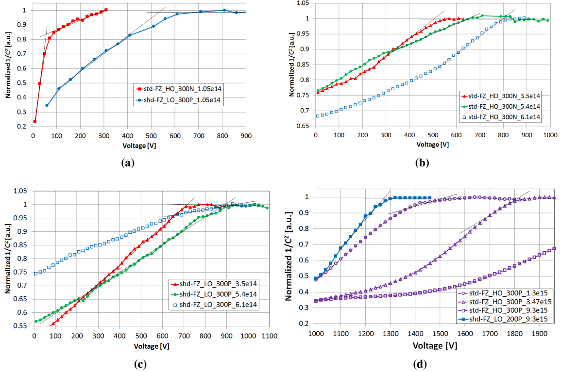
Figure 14. Measured reciprocal C^2 as a function of voltage and extracted V_{fd} -values (crossing point of two linear fits) for (a) 300N/P sensors at (1.05 \pm 0.05) \times 10^{14} \text{ n}_{eq} \text{ cm}^{-2} , (b) 300N sensors and (c) 300P sensors corresponding to figure 13a. Also shown in (d) are the results for 300 \mu\text{m} (300P) and 200 \mu\text{m} (200P) thick n -on- p diodes irradiated up to about 10^{16} \text{ n}_{eq} \text{ cm}^{-2} . Sensor identification and effective fluences (in units of \text{n}_{eq} \text{ cm}^{-2} ) are indicated in the legends.
