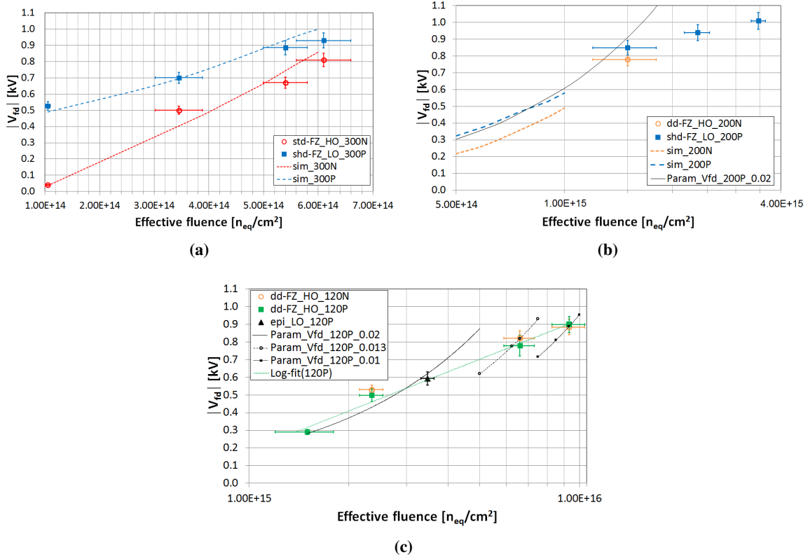
Figure 13. Evolution of full depletion voltage as a function of \Phi_{\text{eff}} for the fluence ranges anticipated for the three sensor thicknesses at HGCal. Simulations are applied up to the neutron defect model’s validated fluence limit [7]. The corresponding CV-curves are presented in figures 14 and 15. (a) Measured (markers) and simulated (dashed curves) V_{\text{fd}}(\Phi_{\text{eff}}) for 300 \mu\text{m} thick sensors. Initial V_{\text{fd}} before irradiation for 300N and 300P were 200 V and 300 V, respectively. (b) Measured and simulated V_{\text{fd}}(\Phi_{\text{eff}}) for 200 \mu\text{m} thick sensors. V_{\text{fd}} before irradiation for 200N and 200P were 95 V and 130 V, respectively. Parametrized V_{\text{fd}}(\Phi_{\text{eff}}) was calculated using eq. (4.5) with standard value of g_{\text{eff}} = 0.02 \text{ cm}^{-1} [24]. (c) Measured V_{\text{fd}}(\Phi_{\text{eff}}) for 120 \mu\text{m} thick sensors. V_{\text{fd}} before irradiation for both 120N and 120P was 50 V, while for epitaxial 120P it was 20 V. Parametrized V_{\text{fd}}(\Phi_{\text{eff}}) was calculated using eq. (4.5) with standard ( 0.02 \text{ cm}^{-1} ), intermediate ( 0.013 \text{ cm}^{-1} ) and saturated ( 0.01 \text{ cm}^{-1} [24]) values of g_{\text{eff}} . The logarithmic fit value for 120P sensors is (0.33 \pm 0.11) \ln(x) - (11 \pm 4) .
