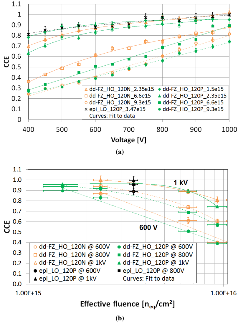
Figure 7. CCE at highest-fluence region as a function of voltage and fluence for 120 \mu\text{m} nominal thickness sensors at -30^\circ\text{C} . Sensor identification is indicated in the legends, as well as effective fluences (in units of n_{\text{eq}} \text{cm}^{-2} ) in panel (a). (a) Measured CCE( V ) with polynomial fits to data. (b) Measured CCE( \Phi_{\text{eff}} ) with corresponding logarithmic and polynomial fits for both dd-FZ sensor polarities.
