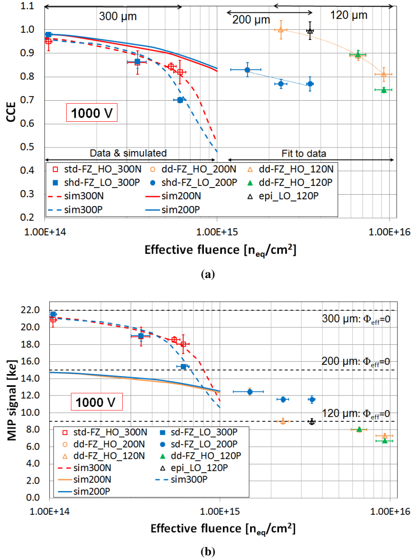
Figure 10. Corresponding CCE and MIP charge collection as a function of fluence to figures 8 and 9 at 1 kV. Sensor identification is indicated in the legends. (a) Measured and simulated CCE(\Phi_{\text{eff}}) with the fluence range of the data points for each sensor thickness indicated. Also indicated, the curves below and above 1 \times 10^{15} \text{ n}_{\text{eq}} \text{ cm}^{-2} are simulated results (thick solid and dashed) and logarithmic (200P) and polynomial (120N) fits to data (thin dotted), respectively. (b) Measured and simulated Q_{\text{coll}}(\Phi_{\text{eff}}) from MIP charge deposition with Q_{\text{coll}} for each active thickness at CCE = 1 indicated [16, 17].
