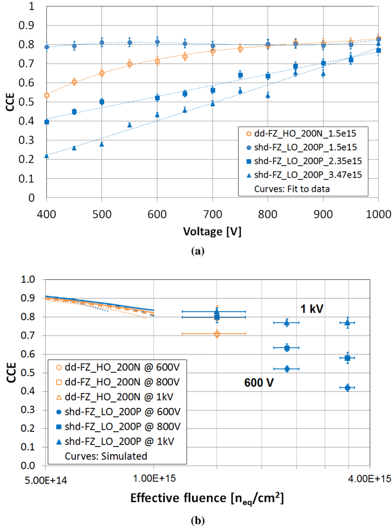
Figure 6. CCE at intermediate-fluence region as a function of voltage and fluence for 200 \mu\text{m} thick sensors at -30^\circ\text{C} . Sensor identification is indicated in the legends, as well as effective fluences (in units of n_{eq} \text{ cm}^{-2} ) in panel (a). (a) Measured CCE( V ) with fits to data (polynomial and linear fits for the two lower-fluence and the two higher-fluence results, respectively) included. (b) Measured and simulated (dotted for 600 V, dashed for 800 V and solid curves for 1 kV) CCE( \Phi_{eff} ).
