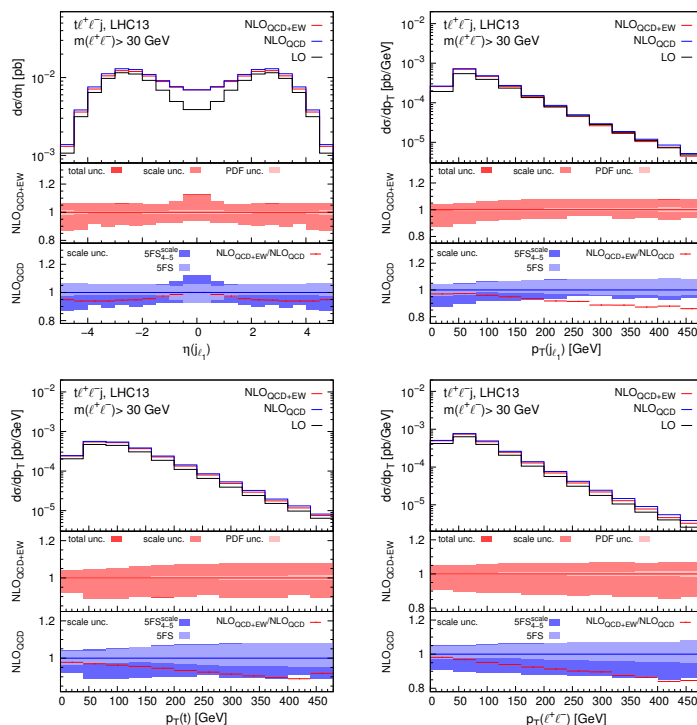
Figure 7. NLO_{QCD+EW} predictions for t\ell^+\ell^-j (“inclusive”). The layout of the plots is the same of figure 4.
