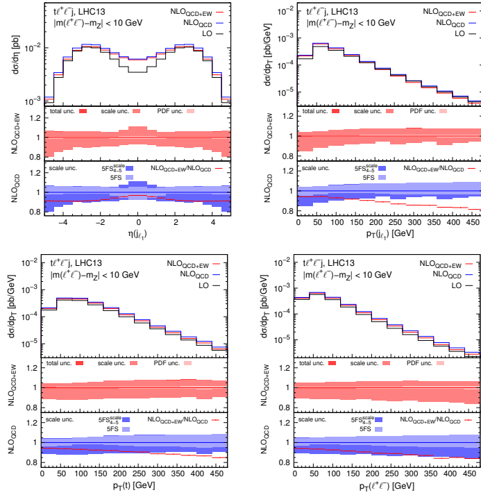
Figure 6. NLO_{QCD+EW} predictions for t\ell^+\ell^-j ( Z -peak). The layout of the plots is the same of figure 4.
