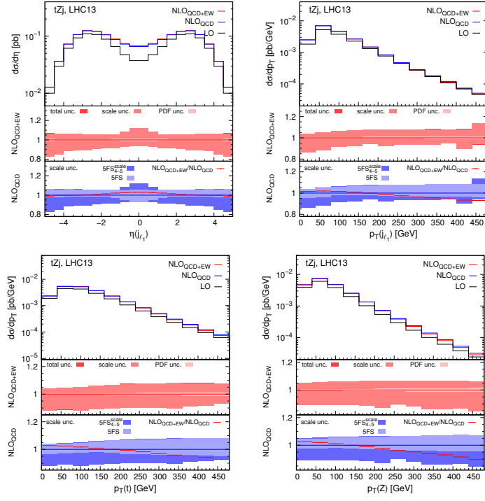
Figure 5. NLO_{QCD+EW} predictions for tZj . The layout of the plots is the same of figure 4.
