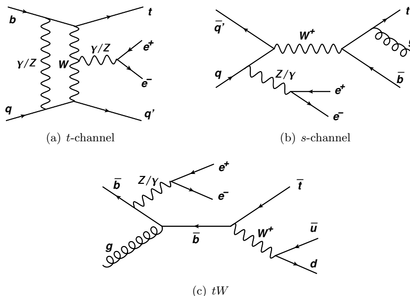
Figure 1. Representative Feynman diagrams for the different channels entering the \text{NLO}_{\text{QCD}+\text{EW}} predictions for t\ell^+\ell^-j production. The diagram 1(a) contributes to the \text{NLO}_2 , while the diagrams 1(b) and 1(c) contribute to the \text{NLO}_1 . Similar diagrams are present for tZj production, while in tHj production the Higgs boson does not couple to the initial-state particles.
