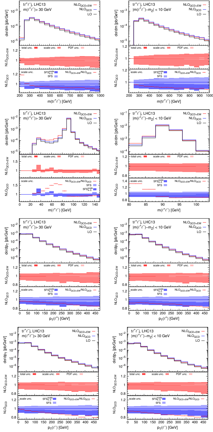
Figure 8. Further plots as in figures 6 and 7 for t\ell^+\ell^-j lepton-based observables. The “inclusive” case is displayed on the left while the Z -peak one on the right.
