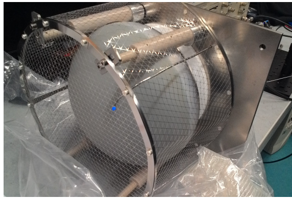
Figure 17. Picture showing the stainless steel pipe which drives the end section of the calibration optical fiber toward the PMT window. A blue-light laser spot on the PMT surface can be noticed.
