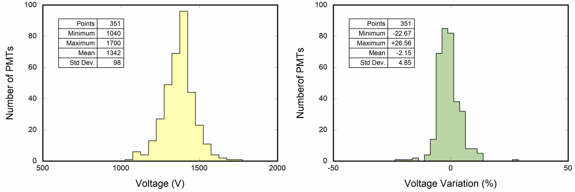
Figure 20. Left: distribution of voltages to attain a gain G = 10^7 for a set of 351 PMTs. Right: distribution of voltage variation (percentage) with respect the calibration performed at CERN [13]. The results are consistent with a standard deviation of about 5%.
