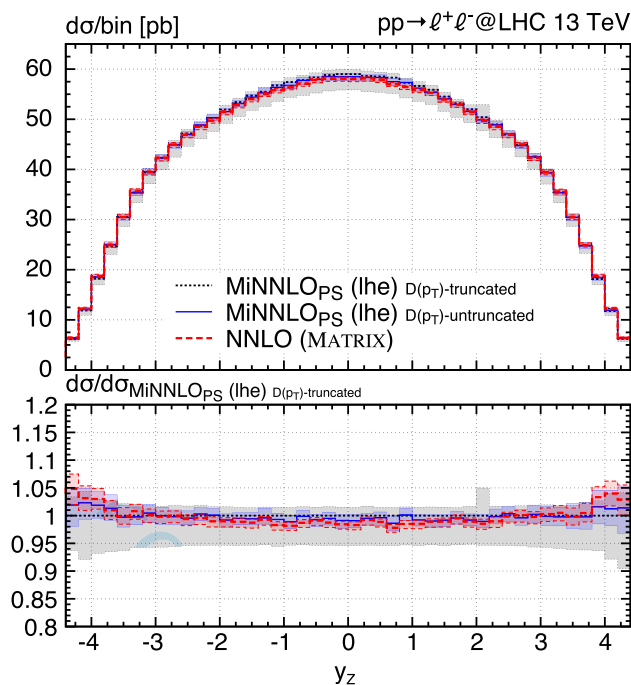
Fig. 1 Rapidity distribution of the Z boson. The plot compares the MiNNLO PS prediction with untruncated (blue solid) and truncated (black dotted) D(p_T) function at the LHE level with the NNLO prediction obtained with MATRIX (red, dashed). The lower panel shows the ratio to the truncated prediction
