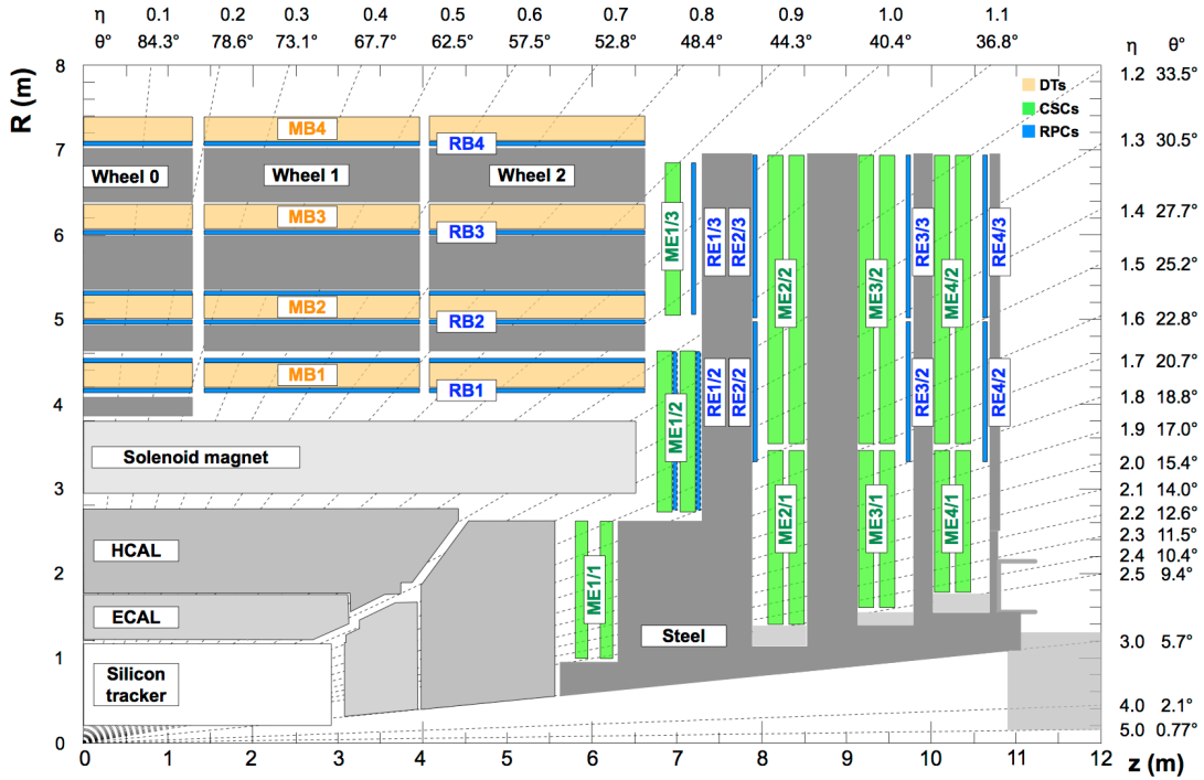
Figure 6: An R - z slice of a quadrant of the CMS detector [15]. The origin of the axes represents the interaction point. The proton beams travel along the z -axis and cross at the interaction point. The three CMS muon subdetectors are shown: four stations of DTs in yellow, labelled MB; four stations of CSCs in green, labelled ME; and four stations of RPCs in blue, labelled RB or RE.
