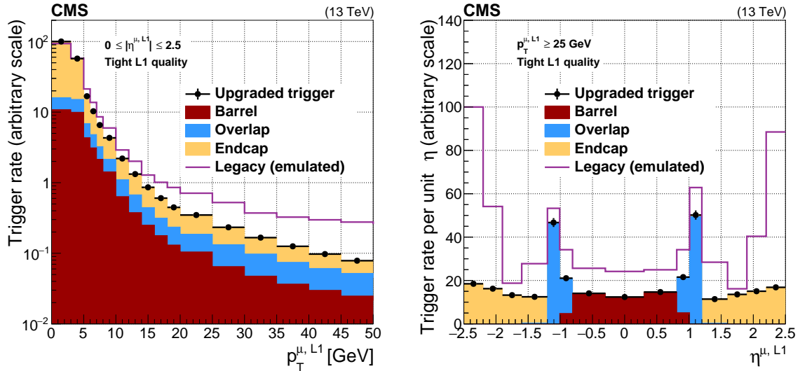
Figure 13: Rates of the re-emulated legacy Run 1 algorithms compared to the upgraded Run 2 algorithms, as a function of the Level-1 muon trigger p_T threshold (left) and \eta (right). The most common Level-1 single-muon trigger threshold used in 2017 was p_T^{\mu, L1} \geq 25 GeV.
