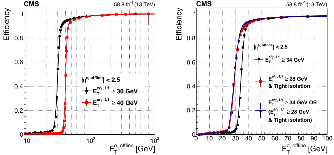
Figure 17: The Level-1 e/\gamma trigger efficiency as a function of the offline reconstructed electron E_T for thresholds of 30 and 40 GeV (left). The Level-1 trigger efficiency as a function of the offline reconstructed electron E_T for two typical unprescaled algorithms used in 2018 (right): an E_T threshold of 34 GeV in black, and of 28 GeV with the tight set of isolation requirements in red (as discussed in the text). The efficiency curve for the logical OR of the two algorithms is shown in blue. The functional form of the fits consists of a cumulative Crystal Ball function convolved with a polynomial or exponential function in the low E_T region.
