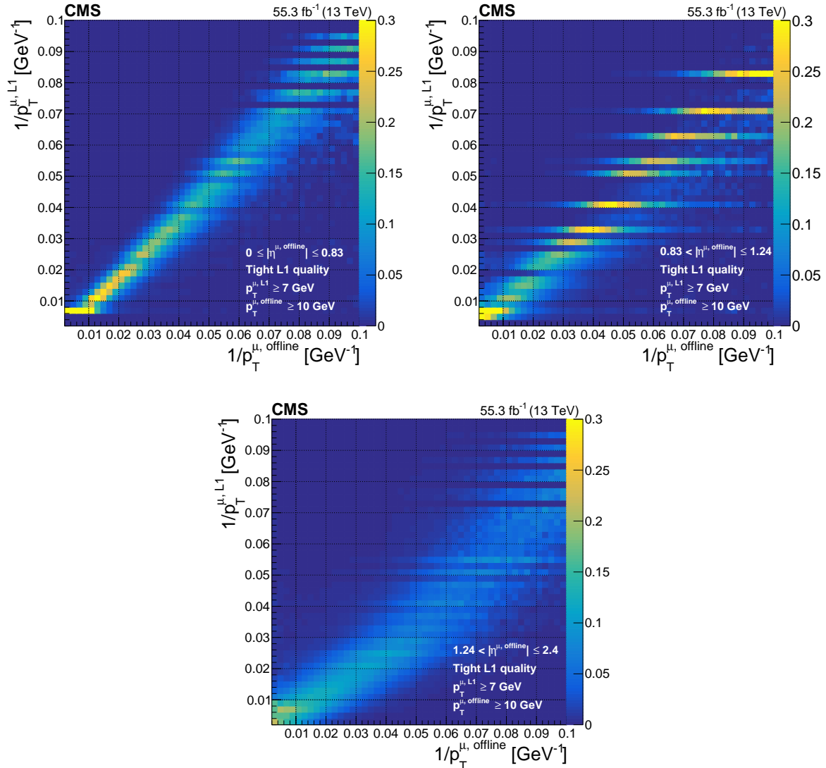
Figure 7: Correlation between 1/p_T of the muon (proportional to curvature) as assigned at Level-1 vs. offline for three |\eta| regions: barrel (top left), overlap (top right), and endcap (bottom). The measurements come from a data set enriched with events with a Z boson. Distinct bands in the overlap region come from more discrete p_T assignment with the OMTF patterns.
