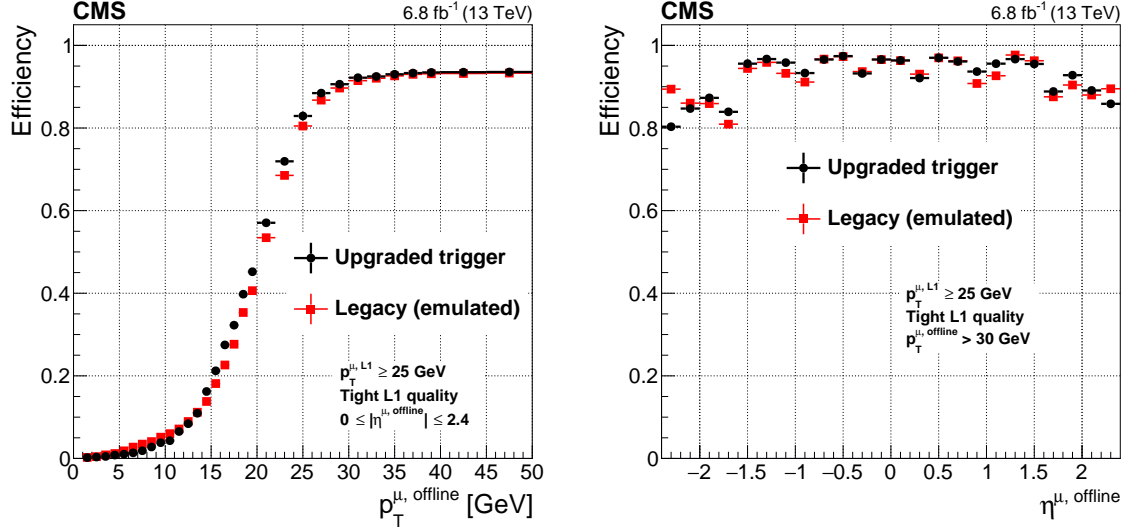
Figure 12: Efficiency of the re-emulated legacy Run 1 algorithms compared with the upgraded Run 2 algorithms, measured using a tag-and-probe technique described in the text, plotted as a function of the offline reconstructed muon p_T (left) and \eta (right). The left figure shows a sharper turn-on efficiency for the upgraded system for muons with p_T between 5 and 25 GeV.
