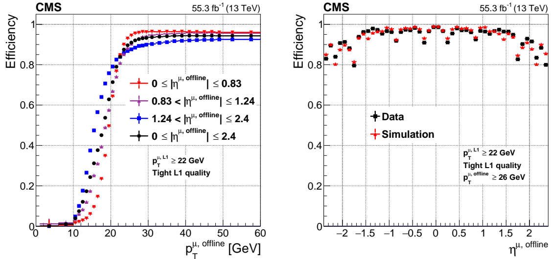
Figure 9: The left plot shows the Level-1 muon trigger efficiency for data as a function of the offline reconstructed muon p_T^{\text{offline}} for each \eta region : barrel region in red, overlap region in purple, endcap region in blue, and the total in black. Turn-on curves for more central muons rise faster primarily because of improved momentum resolution from increased bending in the magnetic field of the yoke. The right plot shows the Level-1 muon efficiency for data and simulation as a function of the offline reconstructed muon \eta . The modulation of the efficiency in \eta is because of the acceptance of the muon systems. The efficiency is measured with the tag-and-probe method described in the text with the full 2018 data set.
