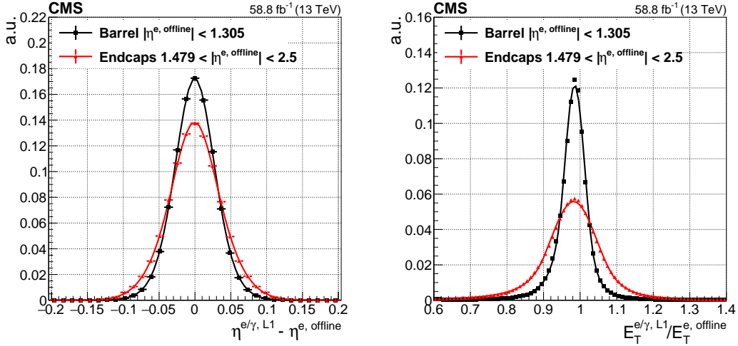
Figure 16: The pseudorapidity position of Level-1 e/\gamma candidates with respect to the offline reconstructed electron position, separately for the barrel and endcap regions (left). The relative transverse energy of the Level-1 e/\gamma candidates with respect to the offline reconstructed electron transverse energy, also separately for the barrel and endcap regions (right). The functional form of the fits consists of a two-sided tail symmetric Crystal Ball function for the left plot and a combination of a Gaussian and an one-sided tail asymmetric Crystal Ball function for the right plot.
