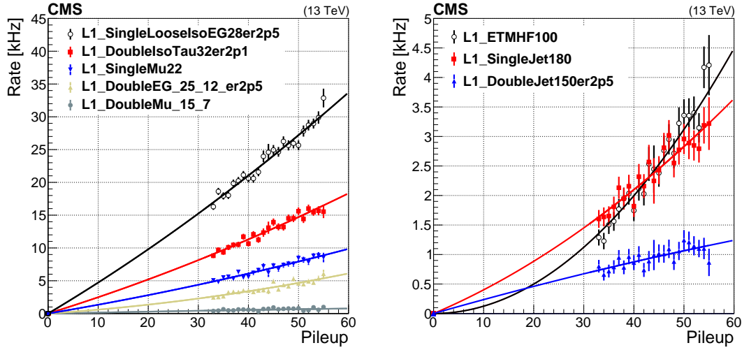
Figure 2: Level-1 trigger rates as a function of pileup for some benchmark seeds targeting leptons (left) and hadrons (right). Rates are measured using data recorded during the 2018 LHC run. Definitions of the seed names are in Table 1. The curves represent fits to the data points that are quadratic and constrained to pass through the origin.
