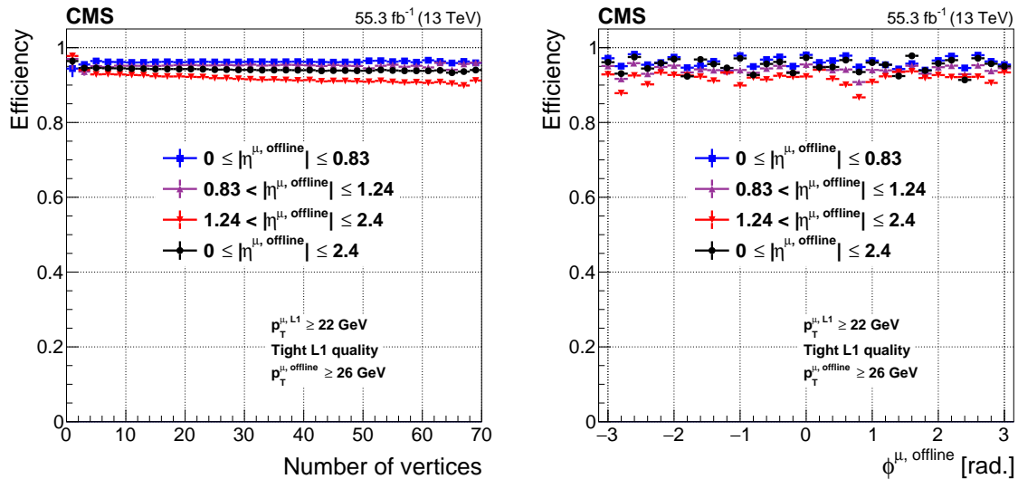
Figure 11: Level-1 trigger efficiency of the muon track finders as a function of the number of offline reconstructed vertices (left) and muon \phi (right), measured with the tag-and-probe method described in the text with the full 2018 data set. These measurements are shown for the most commonly used single-muon trigger threshold in 2018 ( p_T^{\text{L1}} > 22 GeV). The efficiency has no dependence on the number of vertices for central muons, and a very mild dependence for endcap muons. The efficiency modulation in \phi follows the geometrical acceptance of the muon detector: the efficiency is higher in the regions where the detector layers overlap. The efficiency drops at \phi = -2.8 and 0.8 are caused by detector inefficiencies.
