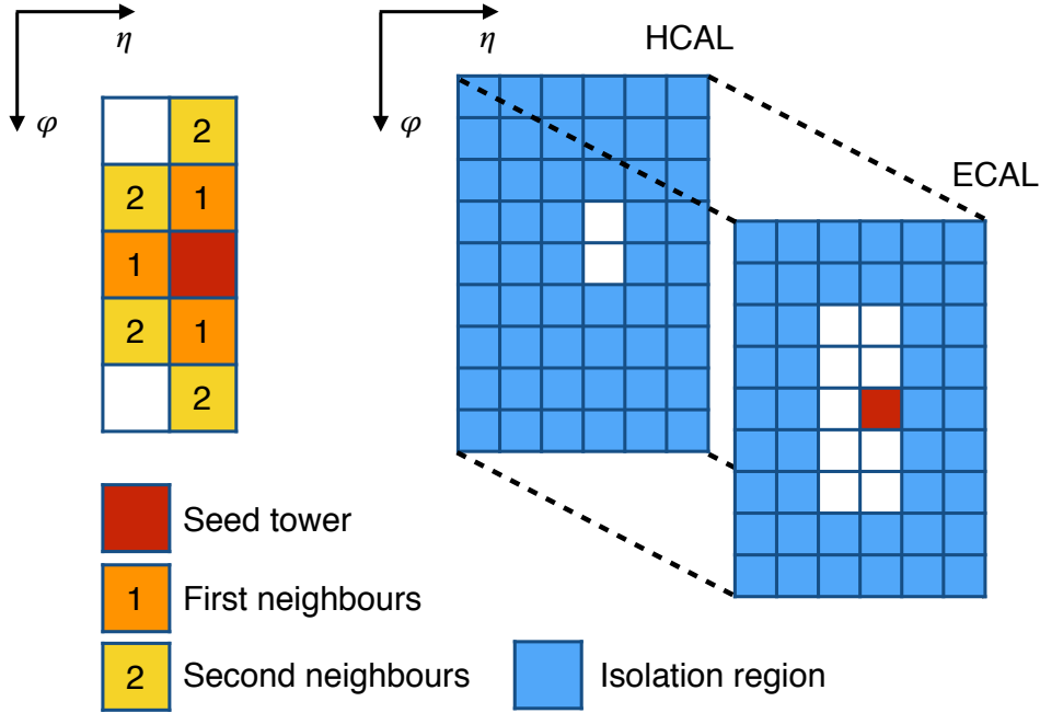
Figure 15: The Level-1 e/\gamma clustering algorithm and isolation definition. A candidate is formed by clustering neighboring towers (orange and yellow) if they can be linked to the seed tower (red). Each square represents a trigger tower. A candidate is considered isolated if the E_T in the isolation region (blue) is smaller than a given value. Details are given in the text.
