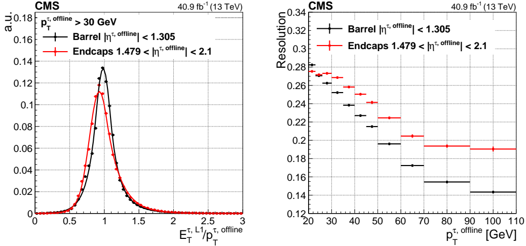
Figure 20: The Level-1 \tau trigger energy response with respect to the offline reconstructed \tau lepton p_T , as measured in 2017 data for the barrel and endcap regions (left). The fits consist of Crystal Ball functions. The resolution as a function of the offline \tau lepton p_T (right), where the resolution is estimated by the root-mean-square of the E_T^{\tau, L1} / p_T^{\tau, \text{offline}} distribution, divided by its mean, in bins of p_T^{\tau, \text{offline}} .
