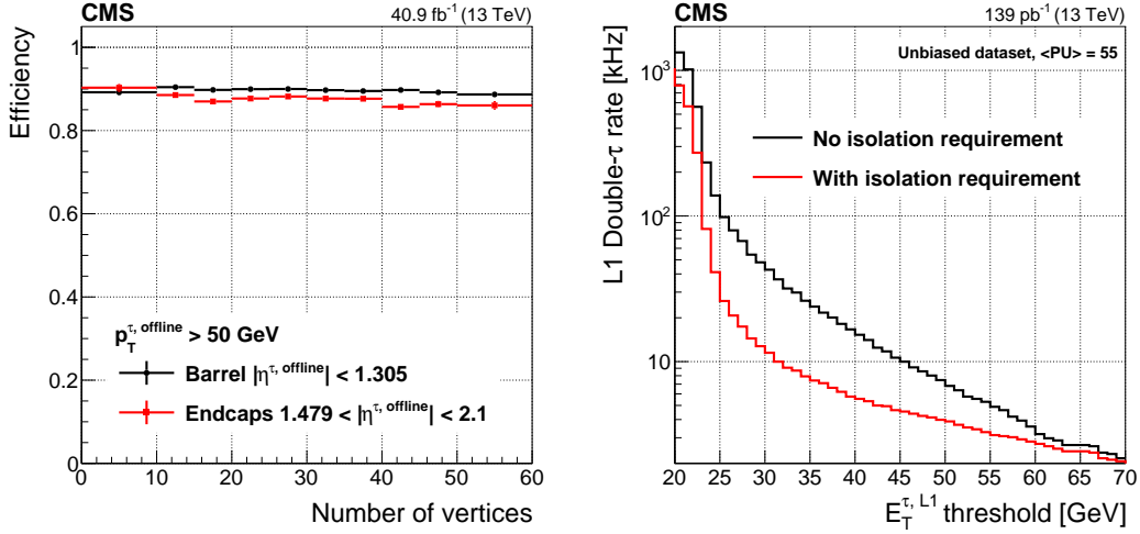
Figure 22: The integrated Level-1 selection efficiency for the isolated \tau trigger with E_T \geq 30 GeV, matched to an offline reconstructed and identified \tau lepton with p_T > 50 GeV, as a function of the number of offline reconstructed vertices (left). The Level-1 double- \tau trigger rate, as a function of the E_T threshold, for \tau candidates with and without an isolation requirement applied (right). The rate is measured requiring two \tau candidates with E_T larger than the bin value, in a unbiased data set with an average pileup of 55.
