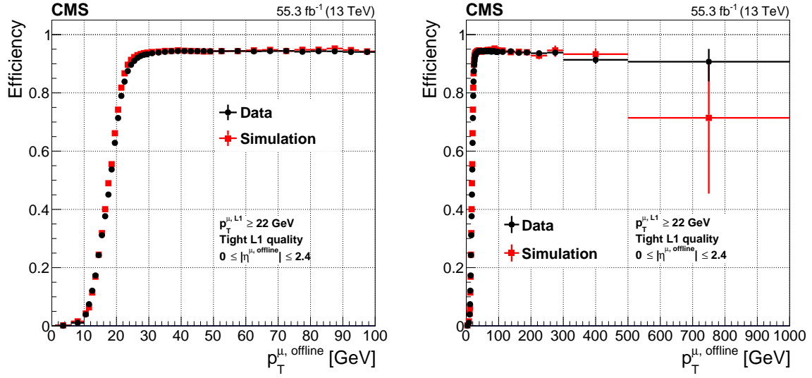
Figure 8: Level-1 trigger efficiency, for data and simulation as a function of p_T^{\text{offline}} , for all reconstructed muons in the CMS acceptance ( |\eta^{\text{offline}}| < 2.4 ) for the most commonly used single-muon trigger during Run 2 ( p_T^{L1} > 22 \text{ GeV} ), measured with the tag-and-probe method described in the text with the full 2018 data set. The left plot focuses on the steep increase part of the curve close to the trigger threshold. The right plot shows the full momentum range up to 1 TeV. The simulation reproduces the data within a few percent accuracy. The Level-1 trigger efficiency plateau is stable as a function of the muon transverse momentum, retaining a high triggering efficiency for muon p_T^{\text{offline}} \leq 1 \text{ TeV} .
