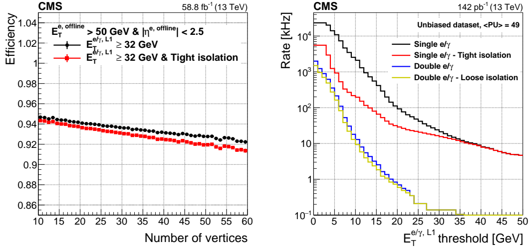
Figure 18: The Level-1 e/\gamma isolated trigger efficiency (left) as a function of the number of offline reconstructed vertices and the Level-1 trigger rate (right) as a function of the E_T threshold applied on the candidate.
