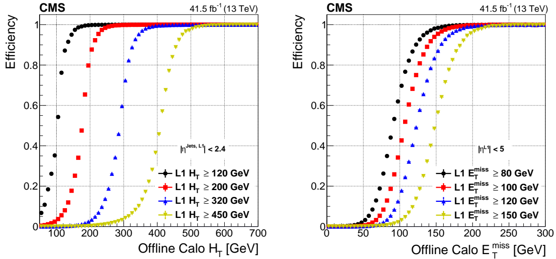
Figure 25: Efficiency curves for the scalar sum of jet energy with E_T \geq 30 GeV (left) and missing transverse energy (right) for various thresholds. The thresholds are indicated as L1 H_T and L1 E_T^{\text{miss}} in the legends.
