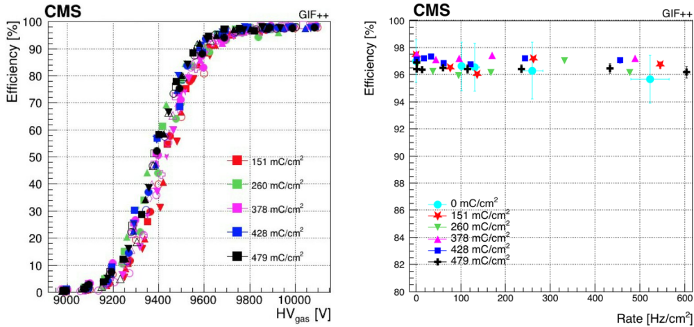
Figure 6. RE2/2 irradiated chamber efficiency as a function of the HV_{gas} (left) at different background irradiation rates and different integrated charge values. The RE2 irradiated chamber efficiency at working point as a function of the background rate at different values of collected integrated charge (right).
