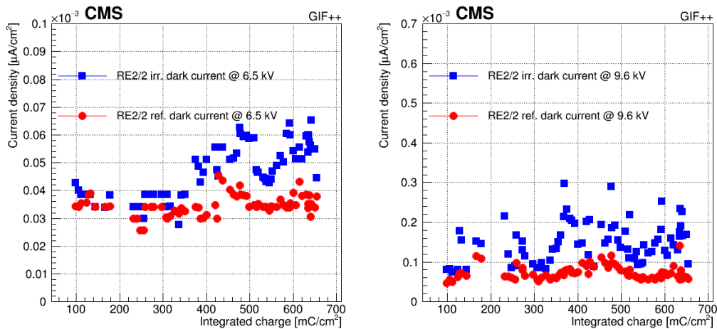
Figure 2. Dark current density for RE2 irradiated (blue squares) and reference (red circles) chambers as a function of collected integrated charge at 6.5 kV (left) and at 9.6 kV (right).
