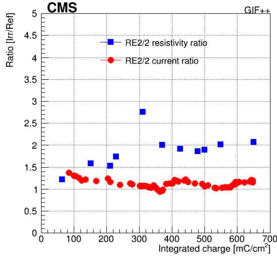
Figure 4. Resistivity ratio (blue squares) and current ratio (red circles) between RE2 irradiated and reference chambers as a function of collected integrated charge.
