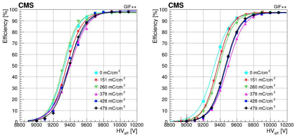
Figure 5. RE2/2 irradiated chamber efficiency as a function of the effective HV, with no irradiation (left) and under a gamma background rate of about 600 Hz/cm 2 (right) at different irradiation periods.
