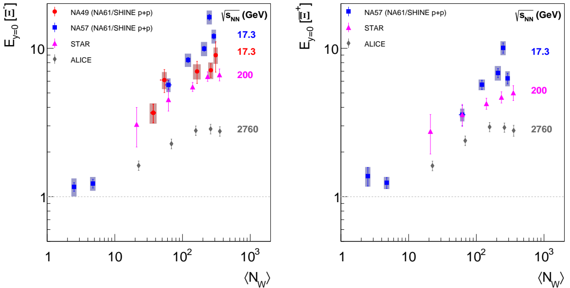
Figure 7: (Color online) The strangeness enhancement E at the mid-rapidity as a function of average number of wounded nucleons \langle N_W \rangle calculated as a ratio of rapidity density for \Xi^- production ( left ) and \Xi^+ production ( right ) in nucleus-nucleus interactions per \langle N_W \rangle divided by the corresponding value for p+p interactions (see Eq. 4). Red circles – NA49 Pb+Pb at 158A GeV [24], blue squares – NA57 p+Be, p+Pb and Pb-Pb at the same center-of-mass energy \sqrt{s_{NN}} = 17.3 GeV [22], magenta triangles – STAR Au+Au at \sqrt{s_{NN}} = 200 GeV [25], gray diamonds – ALICE Pb+Pb at \sqrt{s_{NN}} = 2.76 TeV [26]. The systematic errors are represented by shaded boxes.
