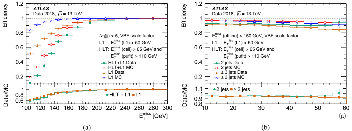
Figure 12: Efficiencies from data and from simulation for L1 (L1XE50) and the combined L1+HLT chain (HLT_xe110_pufit_xe65_L1XE50) triggers are shown for a VBF selection which requires at least two jets that are well separated in rapidity. The uncertainties are statistical only. The lower panels show the ratios between efficiencies in data and simulation. (a) Efficiencies as a function of the offline E_T^{\text{miss}} . In this plot the jet rapidity difference requirement has been tightened to \Delta\eta(\text{jj}) > 5 (b) efficiencies as a function of \langle\mu\rangle for an offline requirement of E_T^{\text{miss}} > 150 GeV using the ‘tenacious’ working point; the efficiencies in data and MC simulation are compared for two different selections, one requiring exactly two and the other \geq 3 jets.
