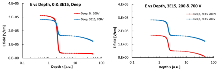
Fig. 8 Effect of irradiation on the electric field in the LGAD with deep gain layer: (left): pre-rad vs. high fluence with bias close to breakdown; (right): low bias vs. high bias for the “Deep” sensor heavily irradiated with neutrons to 3E15 \text{ Neq/cm}^2 .
