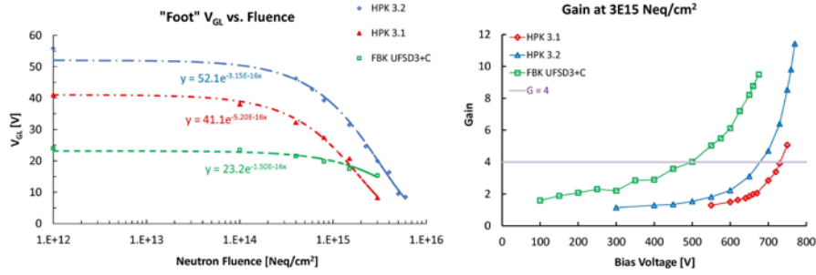
Fig. 6 (left): V_{GL} as a function of neutron fluence for the three selected sensor types; (right): bias dependence of the gain for a neutron fluence of 3E15 , with a gain G = 4 indicated.
