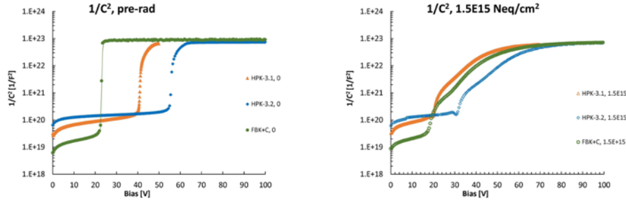
Fig. 5 Measured 1/C^2 vs. bias curves for three selected sensors (left): before irradiation; (right): after a neutron fluence of 1.5E15 \text{ Neq/cm}^2
