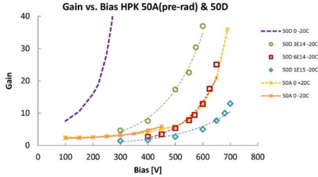
Fig.4 Gain-bias curves for HPK LGAD 50D and 50A pre-rad and 50D after neutron fluences of 3, 6, 10*10 14 Neq/cm 2 .
