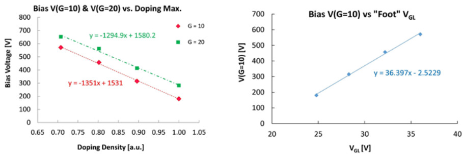
Fig. 3 Correlation between charge collection and doping for the unirradiated HPK prototypes ECX20840: (left): bias V(G=10) and V(G=20) vs. the relative doping density; (right): correlation between V(G=10) and V_{GL} .
