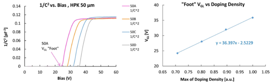
Fig.1 C-V analysis of the HPK prototype ECX20840 before radiation: (left): bias dependence of 1/C^2 to find the bias voltage V_{GL} which depletes the gain layer; (right): correlation between relative doping density and V_{GL} .
