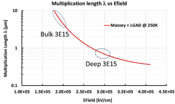
Fig. 9: WF2 simulation [10] of the multiplication length \lambda as a function of electric field following Ref [15]. Both the field achievable in the bulk and in the gain layer are shown for the “Deep” profile after irradiation with 3E15 Neq.
