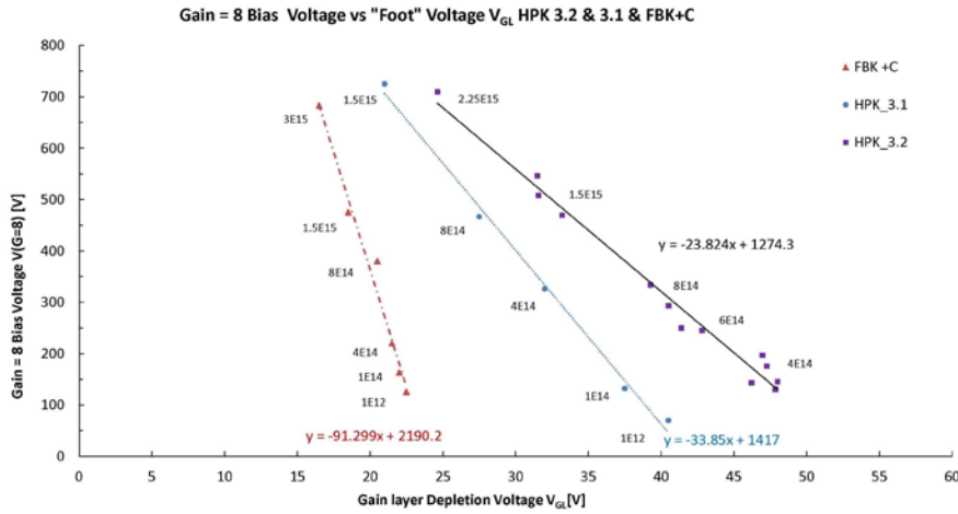
Fig. 10 Correlation between the bias for gain G=8 , V(G=8) , and the “Foot” voltage V_{GL} for the three selected sensors.
