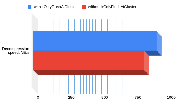
Figure 5. Comparison of decompression speed for two file samples NanoAOD 2017, with and without TTree :: kOnlyFlushAtCluster option.
