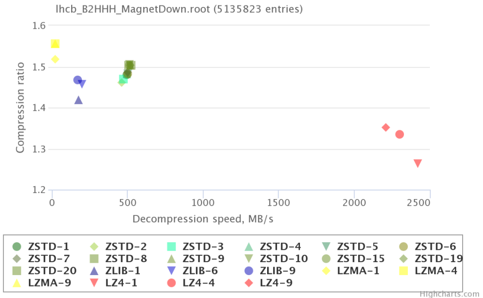
Figure 3. Comparison of compression ratio and decompression speed for all compression algorithms for LHCb file.
