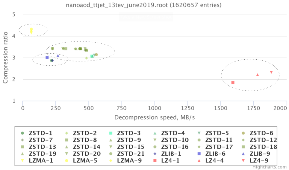
Figure 2. Comparison of compression ratio and decompression speed for all compression algorithms for NanoAOD 2019 file.
