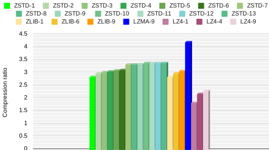
Figure 4. Comparison ratio comparison for custom analysis file with variable-sized data (containing C-style arrays).
