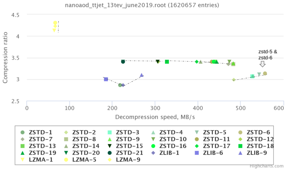
Figure 1. Comparison of compression ratio and decompression speed for ZLIB, LZMA and ZSTD algorithms for NanoAOD 2019 file
