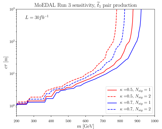
Fig. 2 The expected sensitivities of MoEDAL for various long-lived strongly-interacting sparticle species, assuming 30 fb^{-1} of integrated luminosity. Top panel: the gluino, middle panel: squarks, bottom panel: the stop squark
