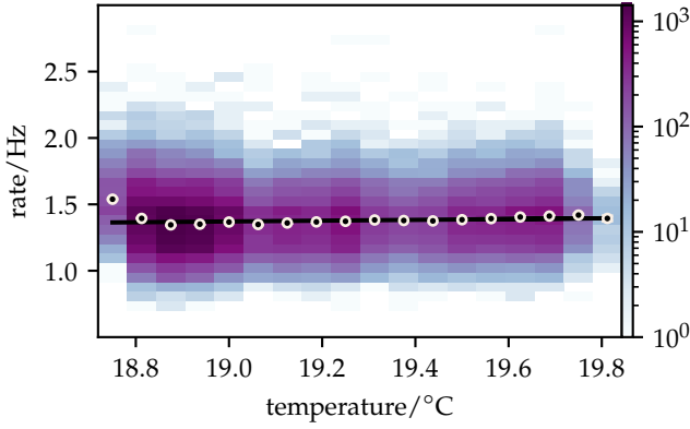
Figure 20. Distribution of the internal-background event-rates in a sealed PMT as a function of the ambient temperature. A linear fit yields a slope of (0.030 \pm 0.014) Hz/°C, which is compatible with our first estimation.
