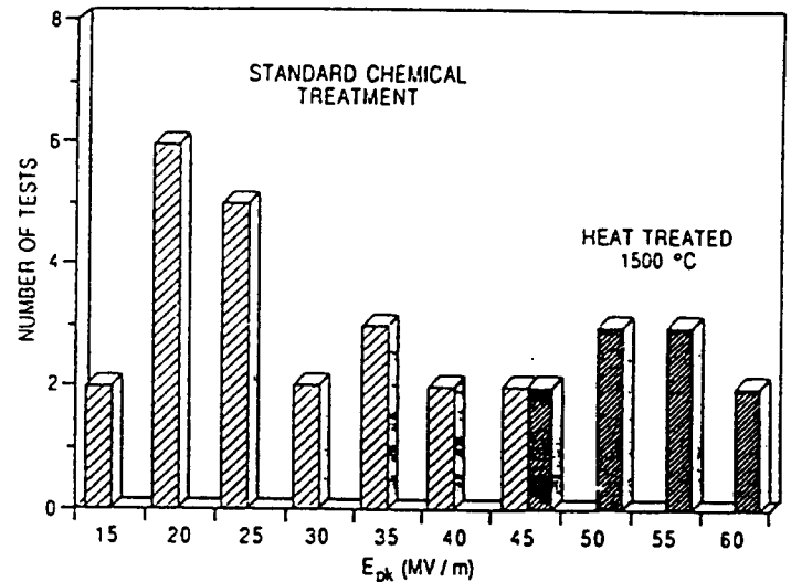
Fig.1. Improvement of cavity performance by heat treatment.
