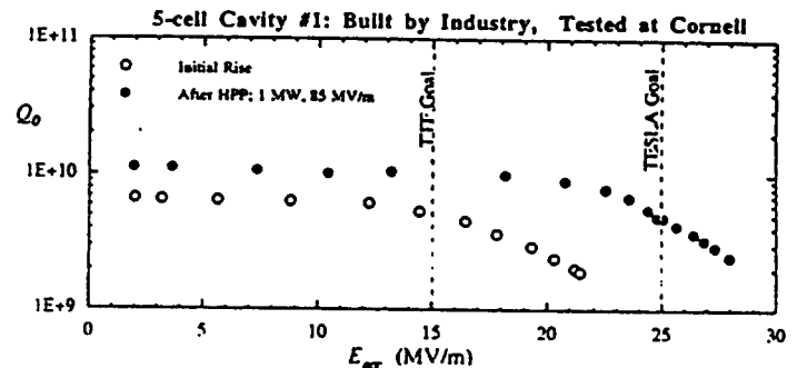
Fig.2. Improvement of cavity performance by HPP.
