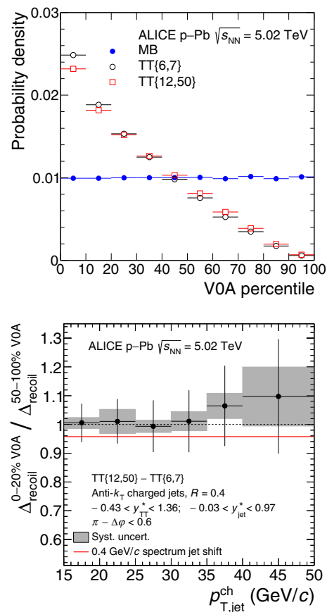
Fig. 5 Figures from Ref. [89]. Top: EA (VOA) distribution for the MB population, and event populations biased by the presence of a high- p_T hadron in the central barrel with 6 < p_T < 7 GeV/c (TT{6, 7}) and 12 < p_T < 50 GeV/c (TT{12, 50}). Decile bins chosen so the MB distribution is uniform. Large VOA amplitude (large EA) corresponds to small VOA percentile. Bottom: Ratio of semi-inclusive recoil jet yield for high and low EA. Red line is the ratio if the high-EA distribution would be shifted to lower p_{T,jet}^{ch} due to p_T -independent energy loss of 400 MeV
