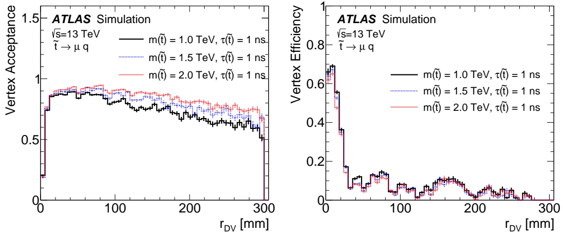
Figure 3: Vertex selection acceptance (left) and efficiency (right) are shown for the \tilde{t} R -hadron benchmark model as a function of the true transverse decay position r_{DV} .
