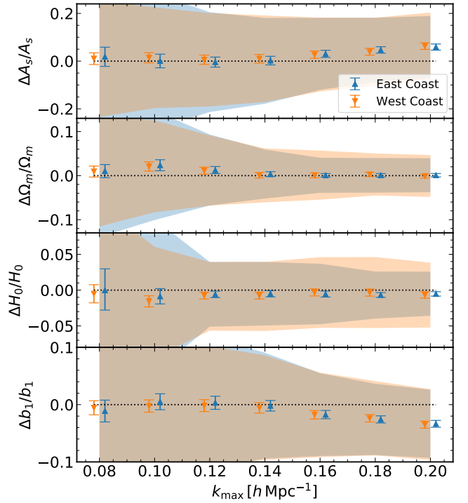
FIG. 7. One dimensional marginalized posterior distributions for the three main cosmological parameters as well as the linear bias parameter as a function of the maximum wavenumber k_{\text{max}} considered in the analysis. The 68% credible intervals derived by the East and West Coast Team are shown respectively by the blue and red error bars with the mean marked by the upward and downward triangles, respectively. Overplotted by the shaded regions are those scaled to the volume of SDSS DR12. The error bars are slightly shifted horizontally to avoid a heavy overlap.
