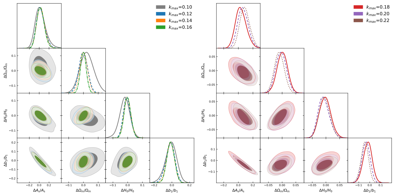
FIG. 13. Expected constraints from a DESI-like survey at different maximum wavenumbers (left: 0.1, 0.12, 0.14 and 0.16 h \text{ Mpc}^{-1} , right: 0.18, 0.2 and 0.22 h \text{ Mpc}^{-1} ). We use the pipeline by the West Coast Team used in the main text for this plot.
