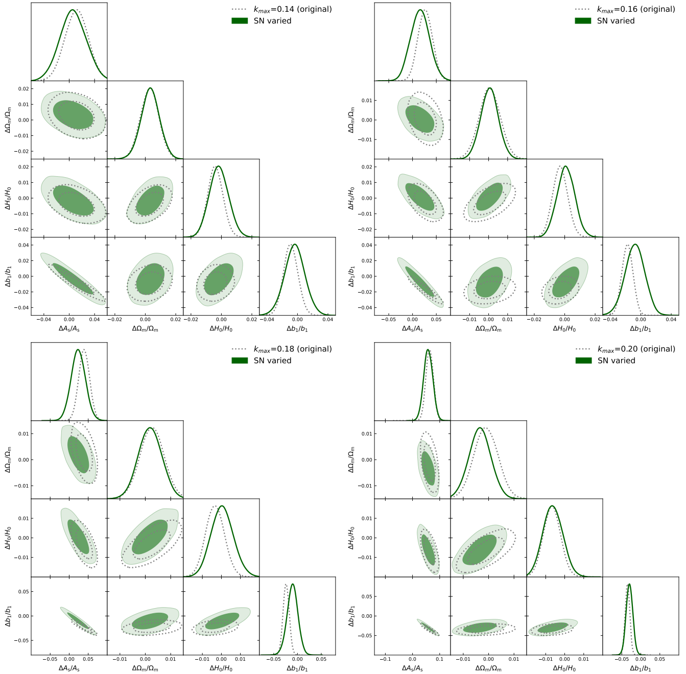
FIG. 12. Similar to Fig. 11, but from the pipeline by the West Coast Team for the case of varied residual shot noise term.
