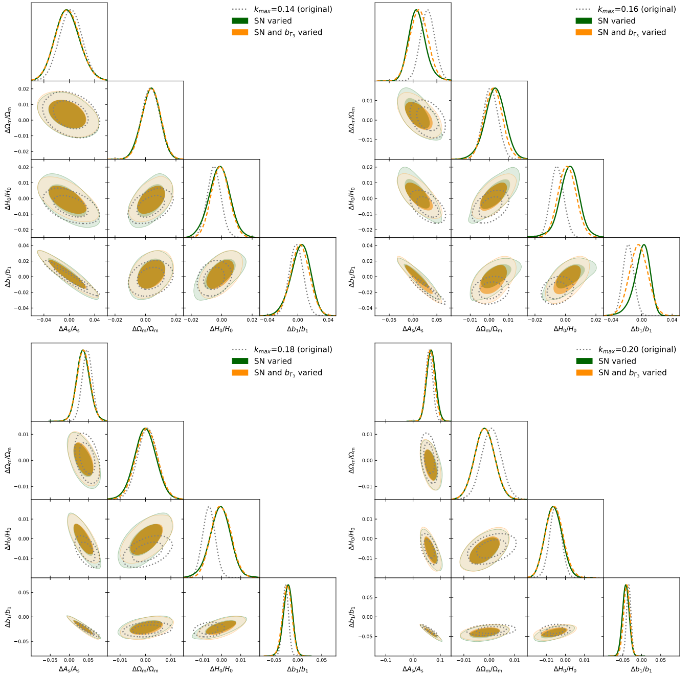
FIG. 11. Posterior distributions from the post-unblinding analyses where one or two additional bias parameters are floated. The results are from the pipeline by the East Coast Team.
