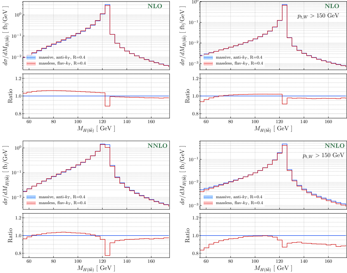
Figure 2: The invariant mass distribution of the two b jets that best reconstruct the Higgs boson mass calculated at NLO (upper plots) and NNLO (lower plots) for central values of the renormalization and factorization scales. Lower panes show ratios of massless to massive results. See text for details.
