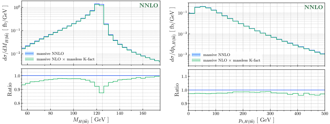
Figure 6: Comparison of approximate and exact NNLO distributions for central values of the renormalization and the factorization scales. Lower panes show ratios of the two distributions with respect to the exact calculation. See text for details.
