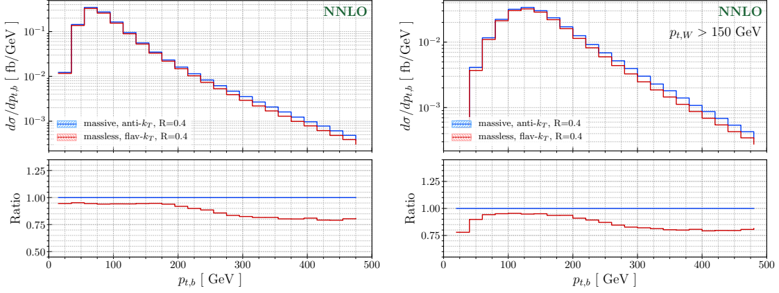
Figure 4: The transverse momentum distribution of the leading b jet calculated at NNLO for central values of the renormalization and factorization scales. Lower panes show ratios of massless to massive results. See text for details.
