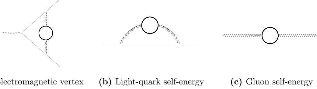
Figure 9: The b -quark contribution to the electromagnetic vertex (a) and to the light quark self-energy (b). In both cases, corrections can be expressed in terms of the b -contribution to the gluon self-energy (c). In this figure, massive quarks are denoted by a thick line. See text for details.
