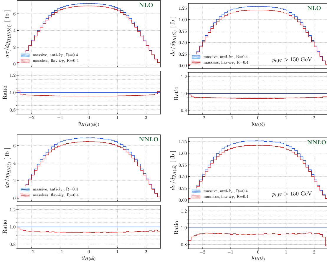
Figure 1: The rapidity distribution of the reconstructed Higgs boson calculated at NLO (upper plots) and NNLO (lower plots) for central values of the renormalization and factorization scales. Lower panes show ratios of massless to massive results. See text for details.
