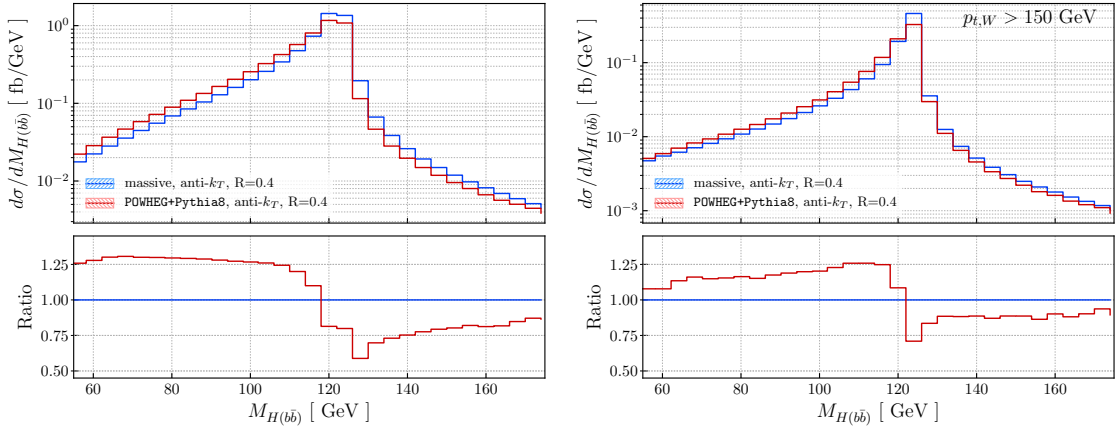
Figure 8: The invariant mass distribution of the two b jets that best reconstruct the Higgs boson mass for central values of the renormalization and factorization scales. Lower panes show ratios of parton shower to massive fixed-order results. See text for details.
