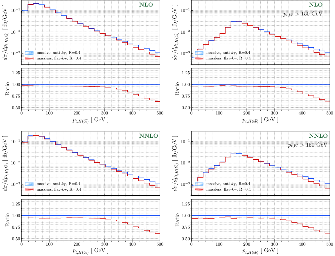
Figure 3: Reconstructed Higgs boson transverse momentum, see text for details, calculated at NLO (upper plots) and NNLO (lower plots) for central values of the renormalization and factorization scales. Lower panes show ratios of massless to massive results. See text for details.
