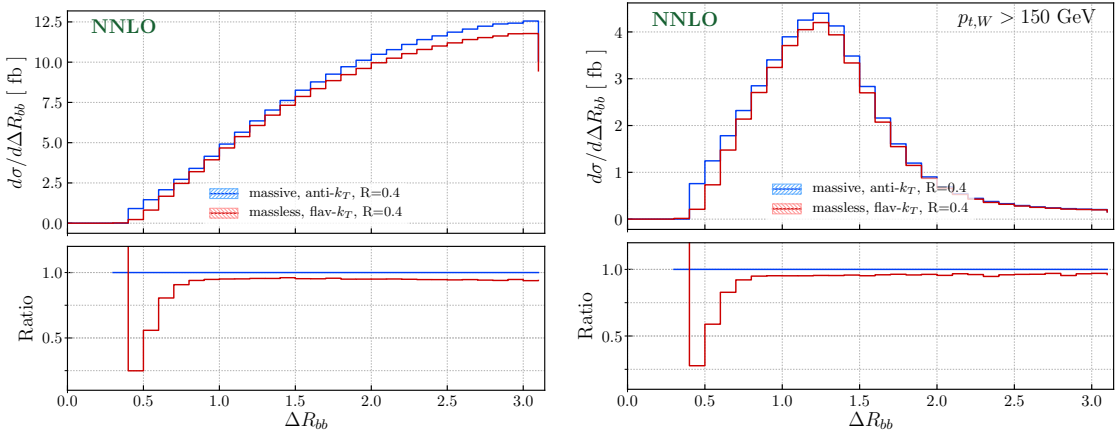
Figure 5: The distance \Delta R_{H(b\bar{b})} between the two b jets used for Higgs boson reconstruction calculated at NNLO for central values of the renormalization and factorization scales. Lower panes show ratios of massless to massive results. See text for details.
