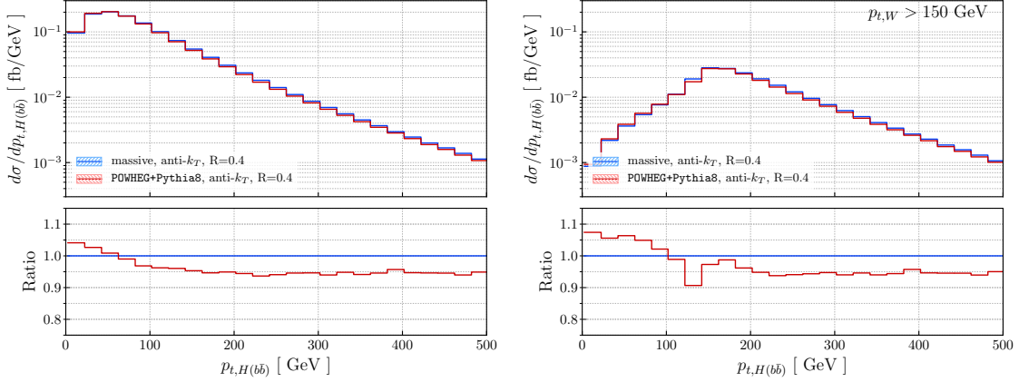
Figure 7: The transverse momentum distribution of two b jets whose invariant mass is closest to the Higgs boson mass for central values of the renormalization and factorization scales. Lower panes show ratios of parton shower to massive fixed-order results. See text for details.
