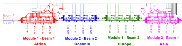
Figure 1: Layout and naming convention of the RF section in the LHC machine as at 14 June 2019.
