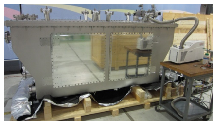
Figure 6: DQW prototype outer vacuum chamber.
