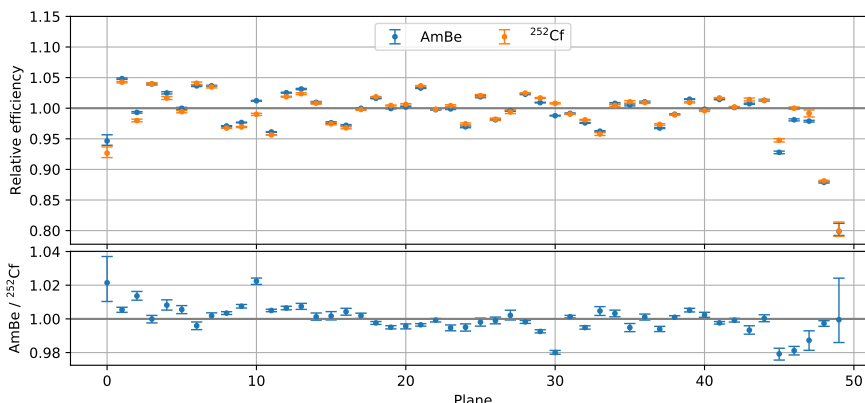
Figure 26. (Top) Relative neutron reconstruction efficiency for the 50 planes obtained with the AmBe (blue) and 252 Cf source (orange). (Bottom) Ratio of the relative neutron reconstruction efficiency obtained with the two different neutrons sources.
