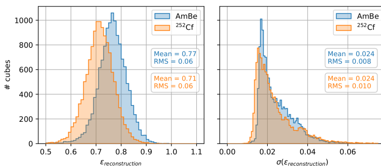
Figure 25. (Left) Neutron reconstruction efficiency for the 12800 cells obtained with the AmBe (blue) and 252 Cf source (orange). (Right) The total uncertainty on the neutron reconstruction efficiency for all detection cells obtained with the two sources (stat. + syst.). The right hand plot shows that the uncertainty is not the same for each cell, which is a consequence of statistics and accessibility during calibration with neutron sources.
