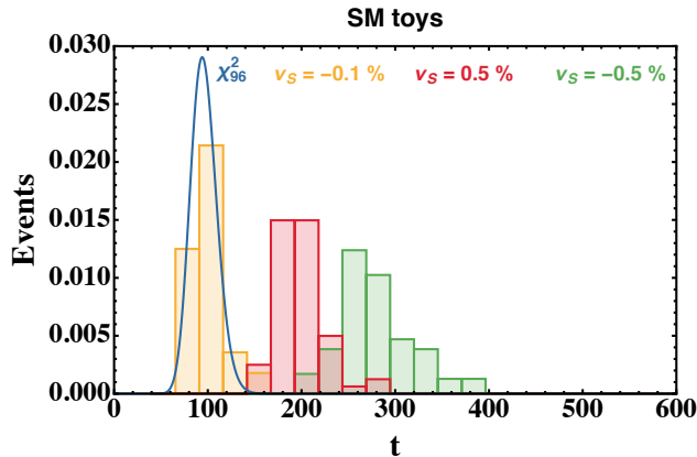
Figure 13: Test statistic distributions for toys generated accordingly to the Standard Model, in the case of -0.1\% (yellow), 0.5\% (red) and -0.5\% (green) mis-calibration of the momentum scale.
