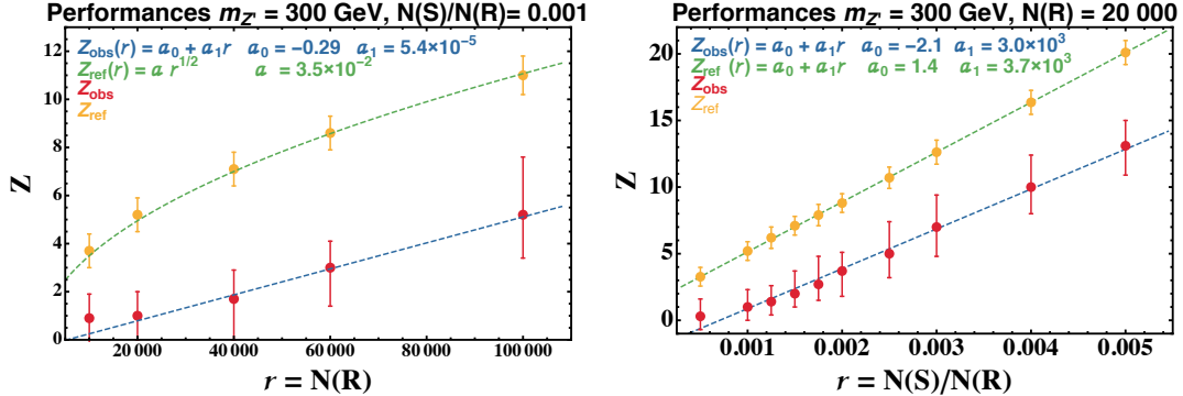
Figure 11: Sensitivity ( Z_{\text{obs}} ) to Z' \rightarrow \mu^+ \mu^- for m_{Z'} = 300 GeV. We show the sensitivity as a function of Luminosity (left panel) and signal fraction (right panel). For reference we plot the reference significance Z_{\text{ref}} and a polynomial fit to the sensitivity.
