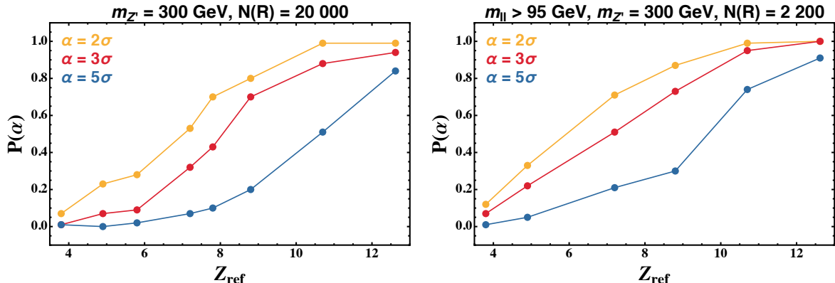
Figure 8: Probability of finding a \alpha = 2\sigma, 3\sigma, 5\sigma evidence for new physics using our technique as a function of the reference significance of the signal, for the Z' model described in Section 4. (Left) Including the Z -peak in the data. (Right) Without the Z -peak.
