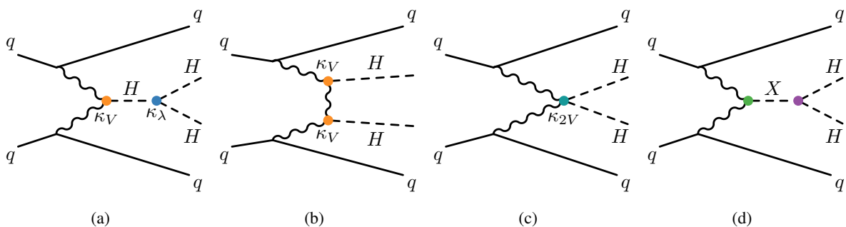
Figure 1: Tree-level Feynman diagrams contributing to Higgs boson pair production via VBF. Diagrams (a), (b) and (c) illustrate the non-resonant production modes scaling with \kappa_V \kappa_\lambda , \kappa_V^2 and \kappa_{2V} , respectively. Diagram (d) illustrates the resonant production mode.
