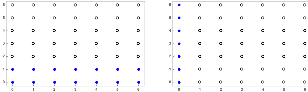
Figure 1: Results for affine Hilbert function h_A(k) in the k = (k_1, k_2) plane (with k_1 on the horizontal axis and k_2 on the vertical axis) for Example 3 with n_C = 3 (left) and Example 4 with n_C = 2 (right). Blue points indicate degrees for which h_A(k) < n_C and empty points satisfy h_A(k) = n_C .
